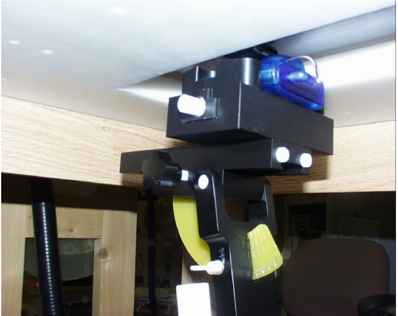
Figure 7. Body Worn Position of the Phone with the Phone clip Placed Under a Flat Phantom
