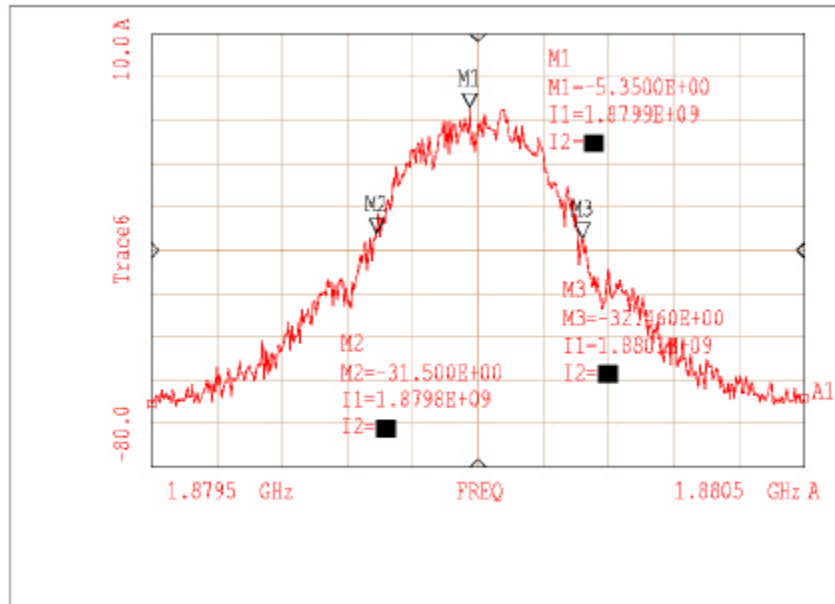
Figure 6E.5 Channel 661, -26dBc Bandwidth
