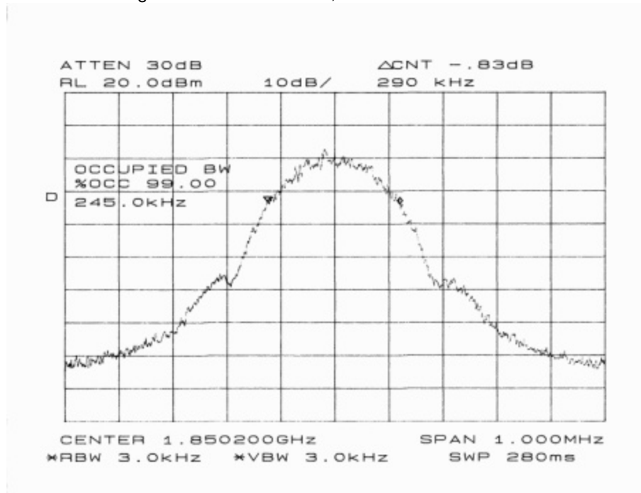
Figure 6E.1 Channel 512, 99% Power Bandwidth
