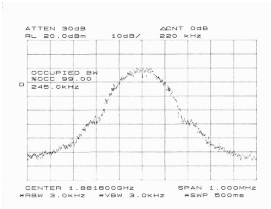
Figure 6E.2 Channel 670, 99% Power Bandwidth
