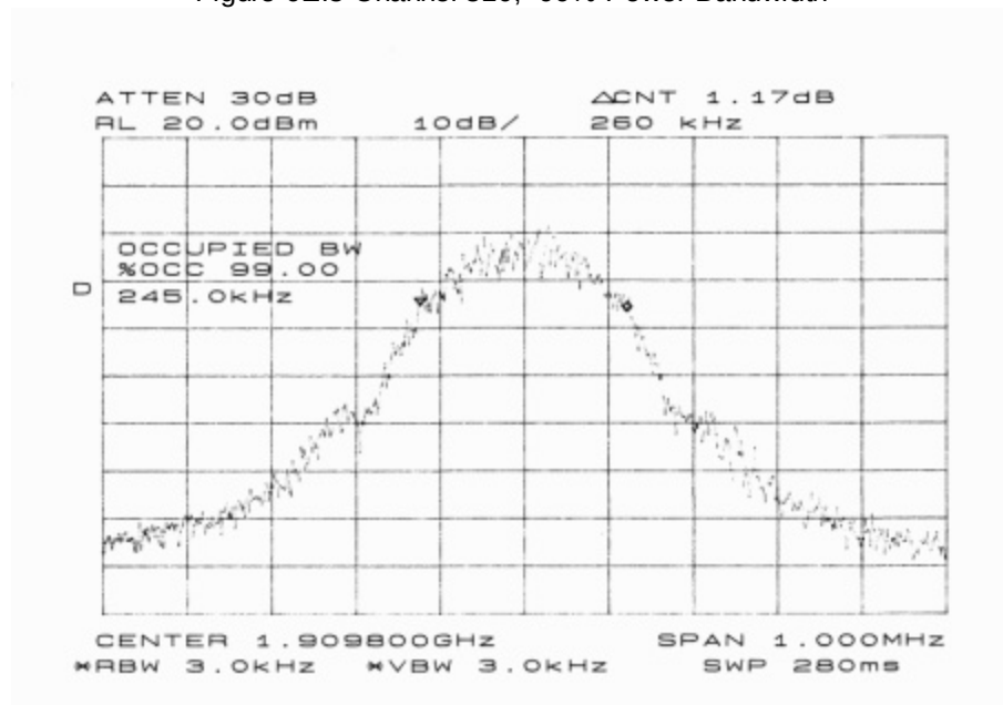
Figure 6E.3 Channel 810, 99% Power Bandwidth
