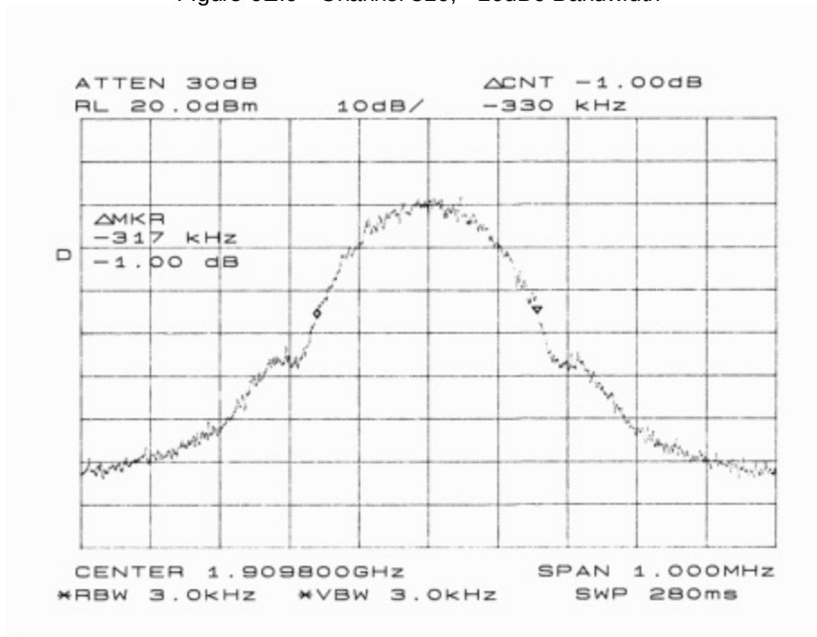
Figure 6E.6 Channel 810, -26dBc Bandwidth
