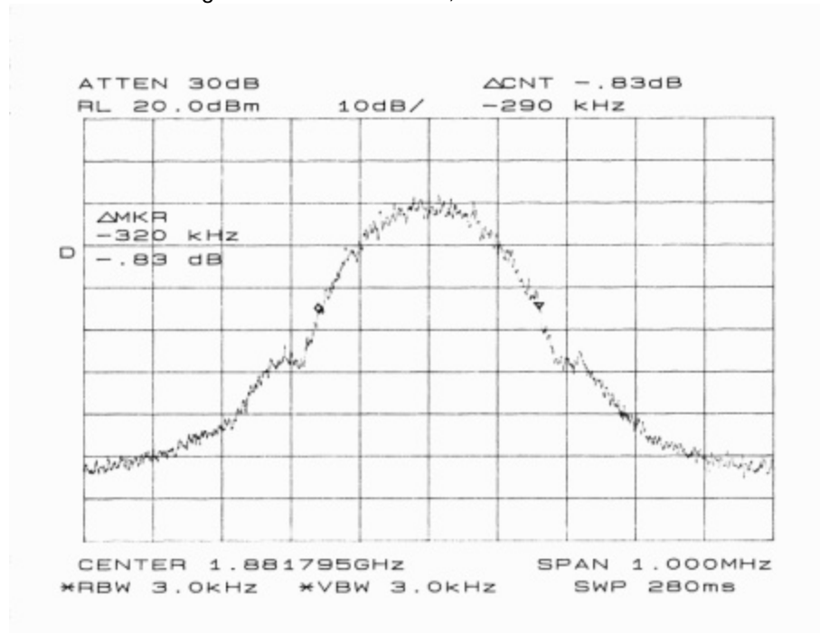
Figure 6E.5 Channel 670, -26dBc Bandwidth
