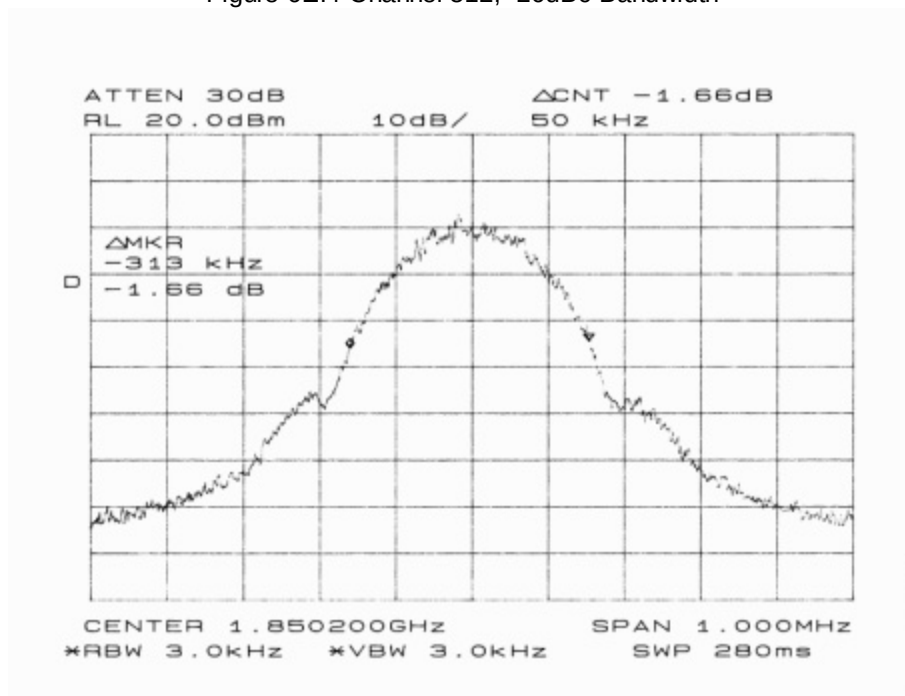
Figure 6E.4 Channel 512, -26dBc Bandwidth
