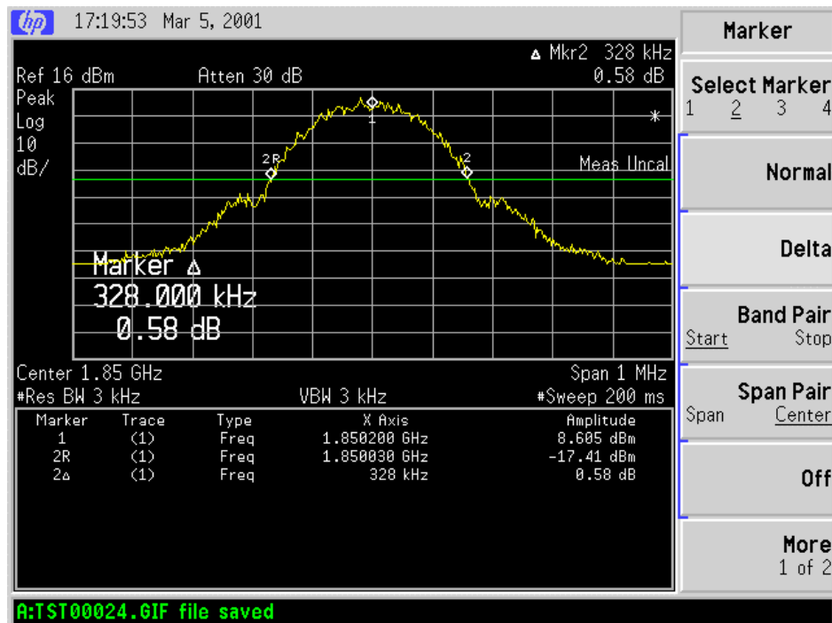
Figure 6E.2 Channel 512, -26dBc Bandwidth
