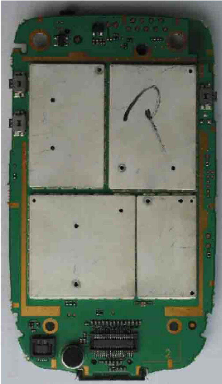
Front View
