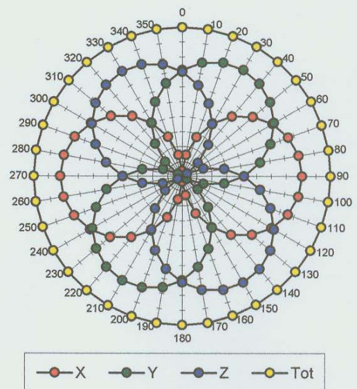
f = 2500 \text{ MHz, WG R22}
