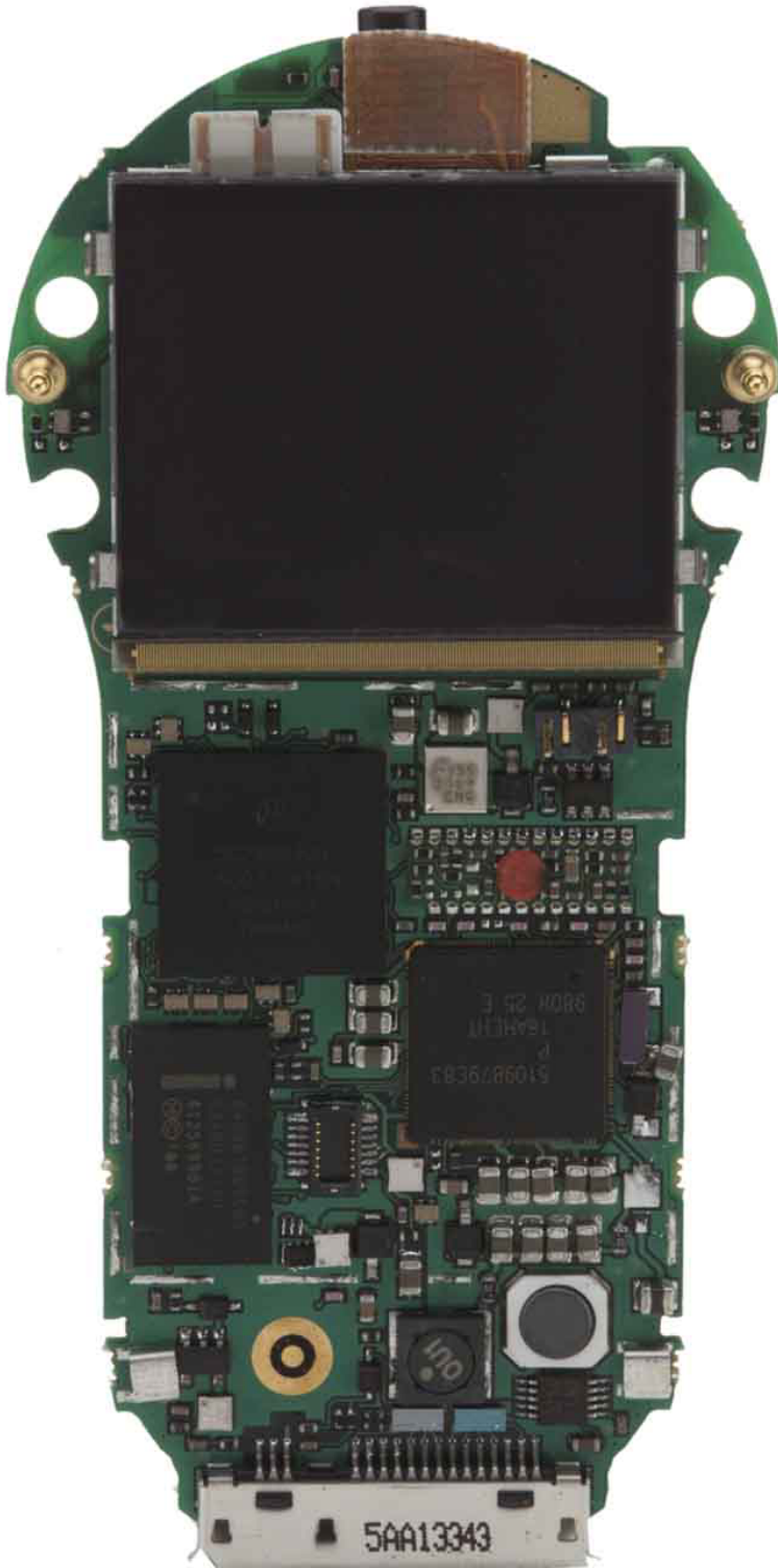
Front View (Shields Removed)
