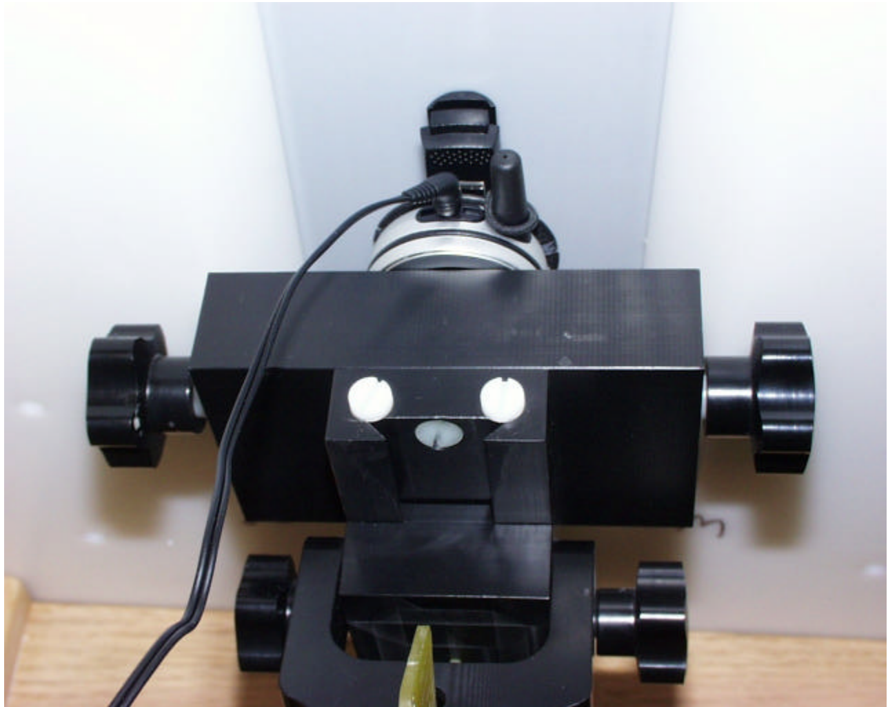
Figure 11. Phone inside (Leather Holster / Belt Clip) under the Flat Phantom with the Head Set Attached
