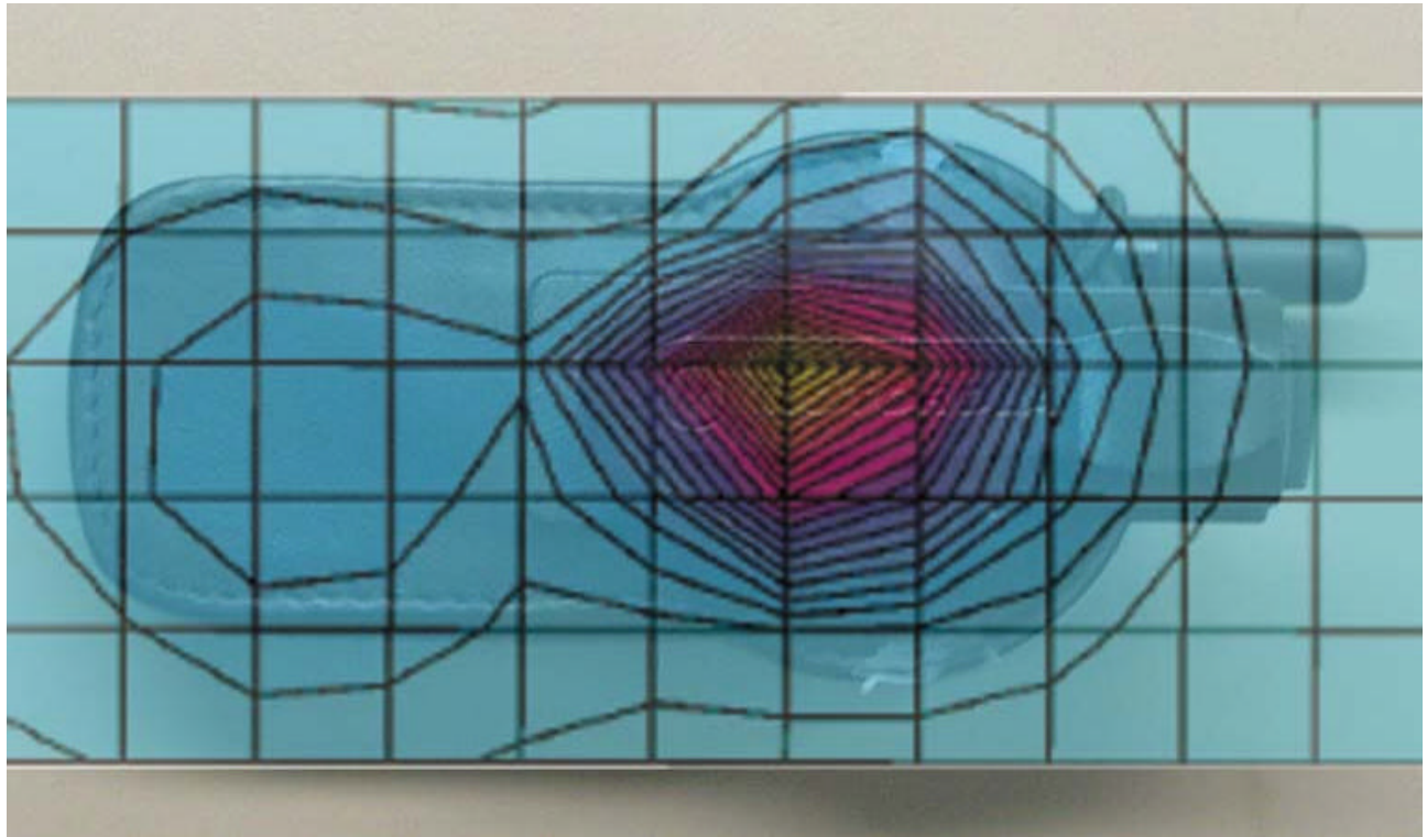
Figure 3. Typical 1900 MHz Body Worn Contour Overlaid with Antenna Fixed
