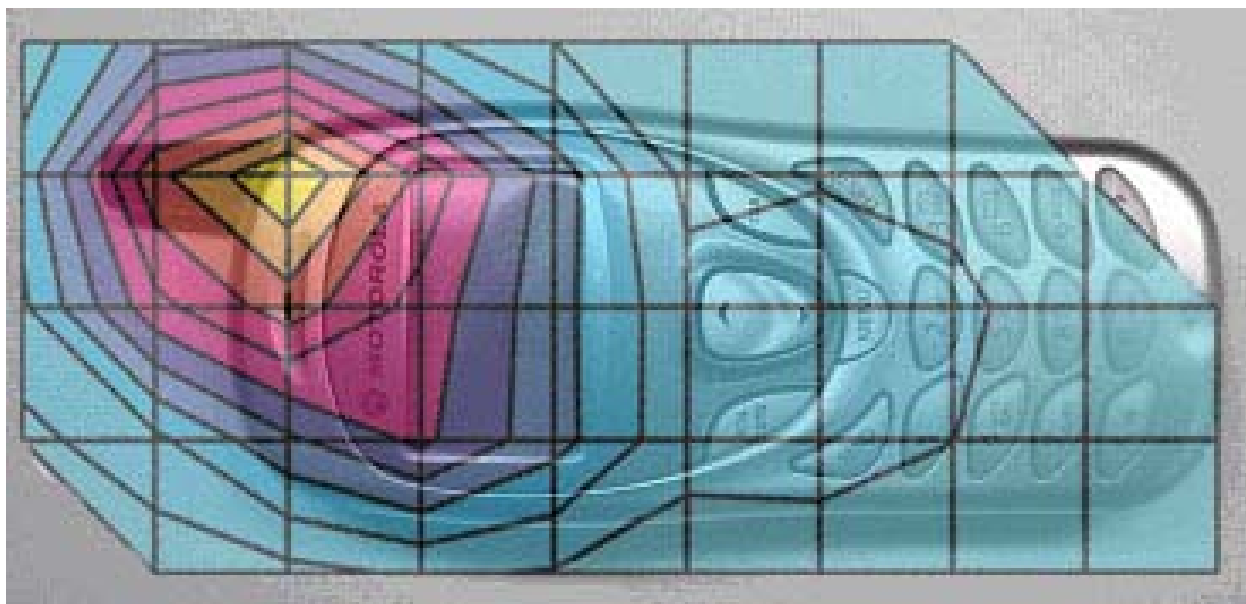
Figure 1. Typical 1900MHz Head Adjacent Contour Overlaid on Phone with Antenna Fixed (Cheek Touch)
