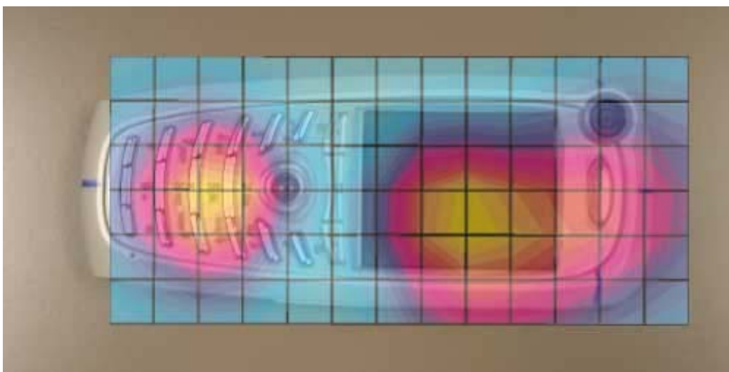
Figure 4. Typical 1900 MHz Body-Worn Contour Overlaid on Phone (Front 1" away)
