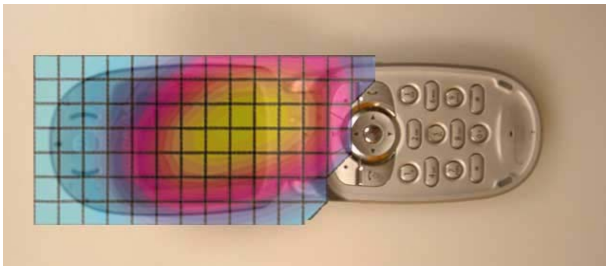
Figure 2. Typical 850 MHz Right Head Adjacent Contour Overlaid on Phone with Antenna Fixed (15° Tilt position)
