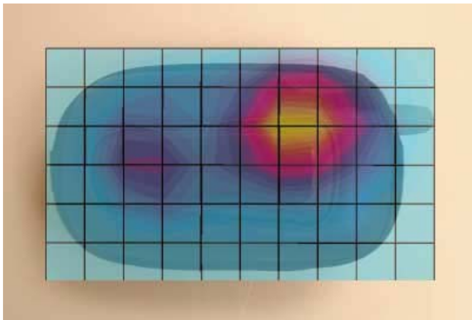
Figure 7. Typical 1900 MHz Body-Worn Contour Overlaid on Phone with Mercury Eva Pouch
