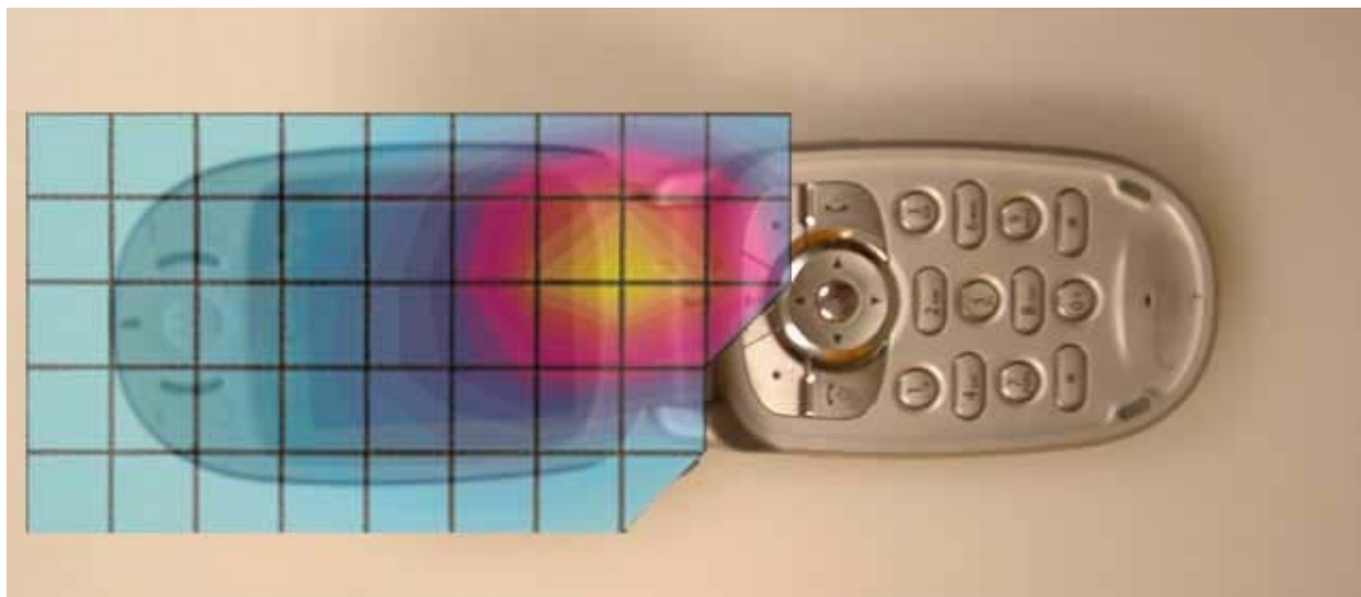
Figure 1. Typical 850 MHz Right Head Adjacent Contour Overlaid on Phone with Antenna Fixed (Cheek Touch)
