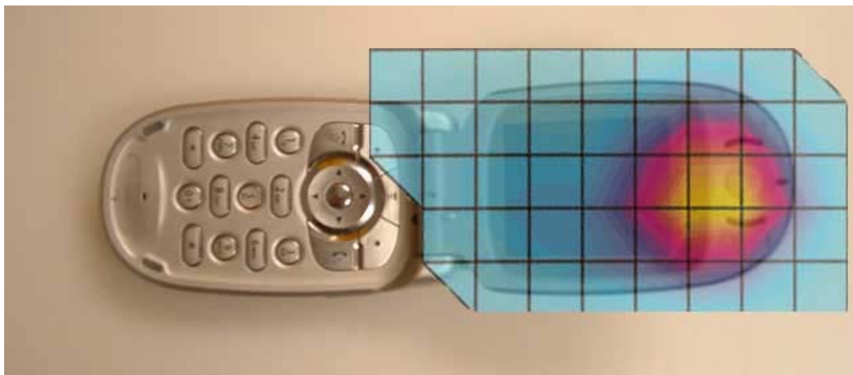
Figure 4. Typical 1900MHz Left Head Adjacent Contour Overlaid on Phone with Antenna Fixed (15° Tilt position)
