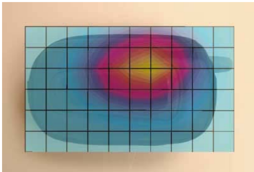
Figure 5. Typical 850 MHz Body-Worn Contour Overlaid on Phone with Mercury Eva Pouch
