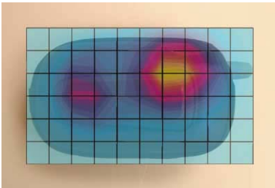
Figure 8. Typical 1900 MHz Body-Worn Contour Overlaid on Phone with Mercury Eva Pouch (GPRS enabled)
