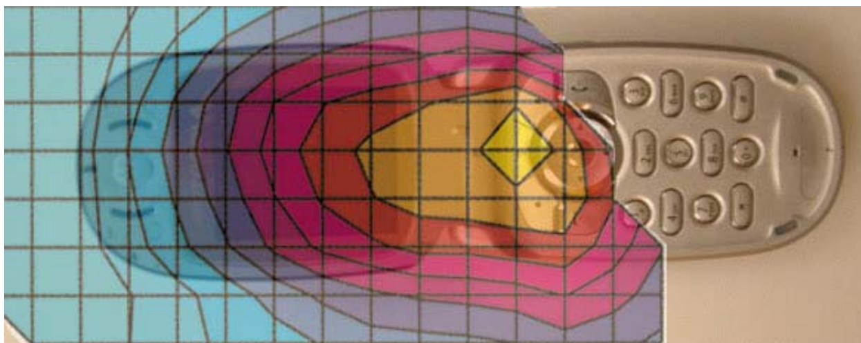
Figure 2. Typical 850 MHz Head Adjacent Contour Overlaid on Phone (15° Tilt position)
