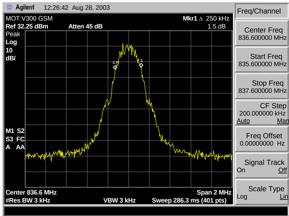
850 GSM Occupied Band
