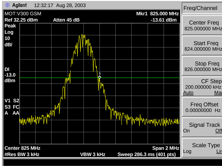
GSM 850 A*(Lower) Max Block Edge
