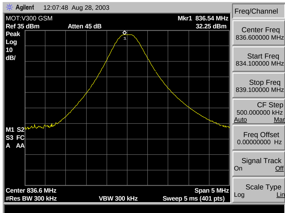
850 GSM Reference Plot
