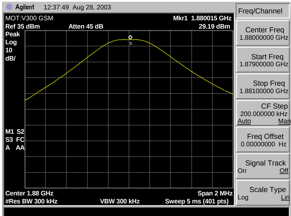
1900 GSM Reference Plot
