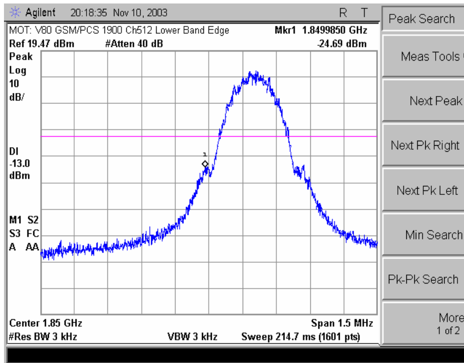
1900 GSM Lower Band Edge
