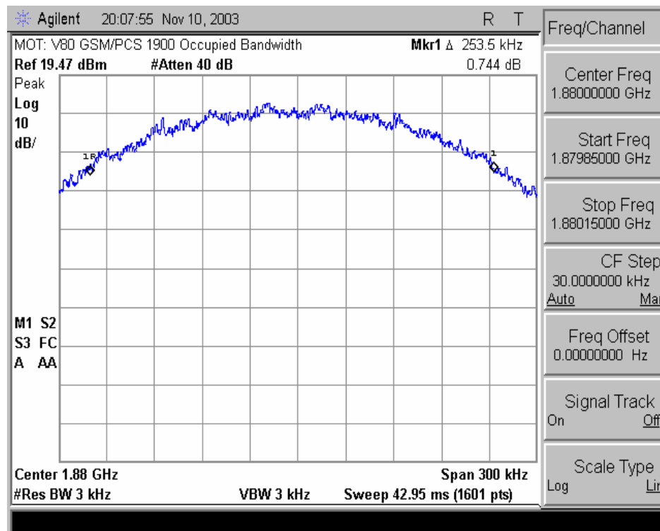
1900 GSM Occupied Bandwidth
