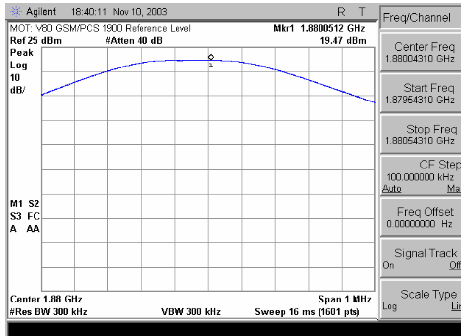
1900 GSM Reference Level
