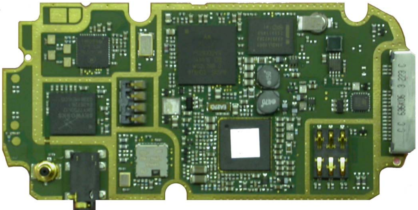
Rear view (shields removed)
