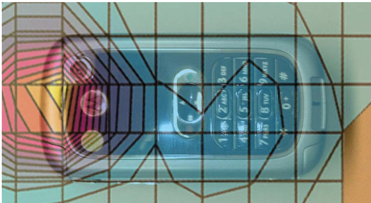
Figure 2. Typical 1900MHz Head Adjacent Contour Overlaid on Phone (15 ° Tilt)
