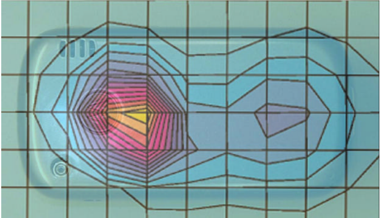
Figure 3. Typical 1900 MHz Body-Worn Contour Overlaid on Phone
