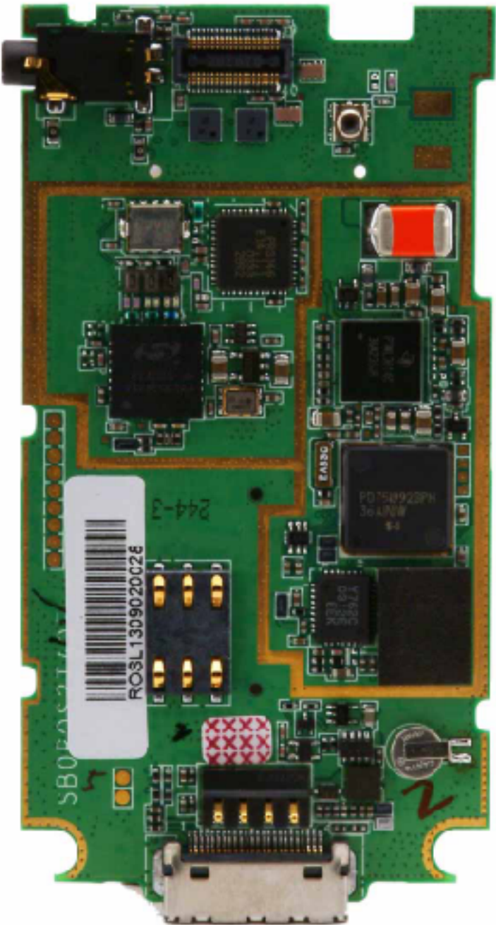
Rear View
