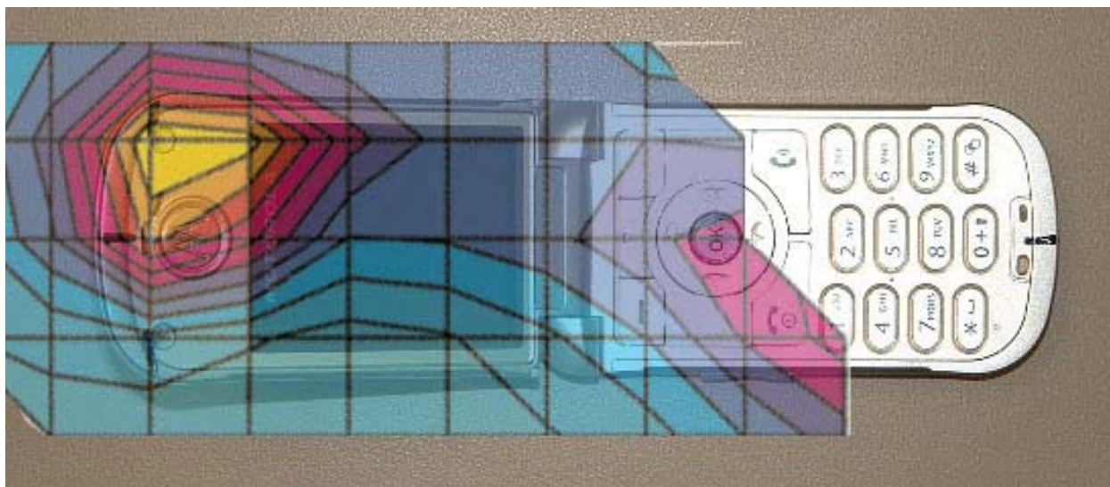
Figure 2. Typical 1900MHz Left Head Adjacent Contour Overlaid on Phone (15 ° Tilt)
