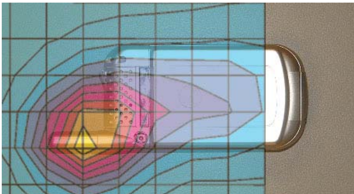
Figure 4. Typical 1900 MHz Body-Worn Contour Overlaid on Phone (GPRS Mode)
