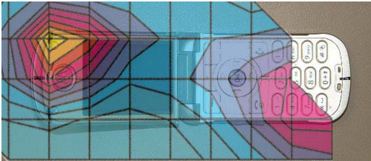
Figure 2. Typical 1900MHz Left Head Adjacent Contour Overlaid on Phone (15 ° Tilt)
