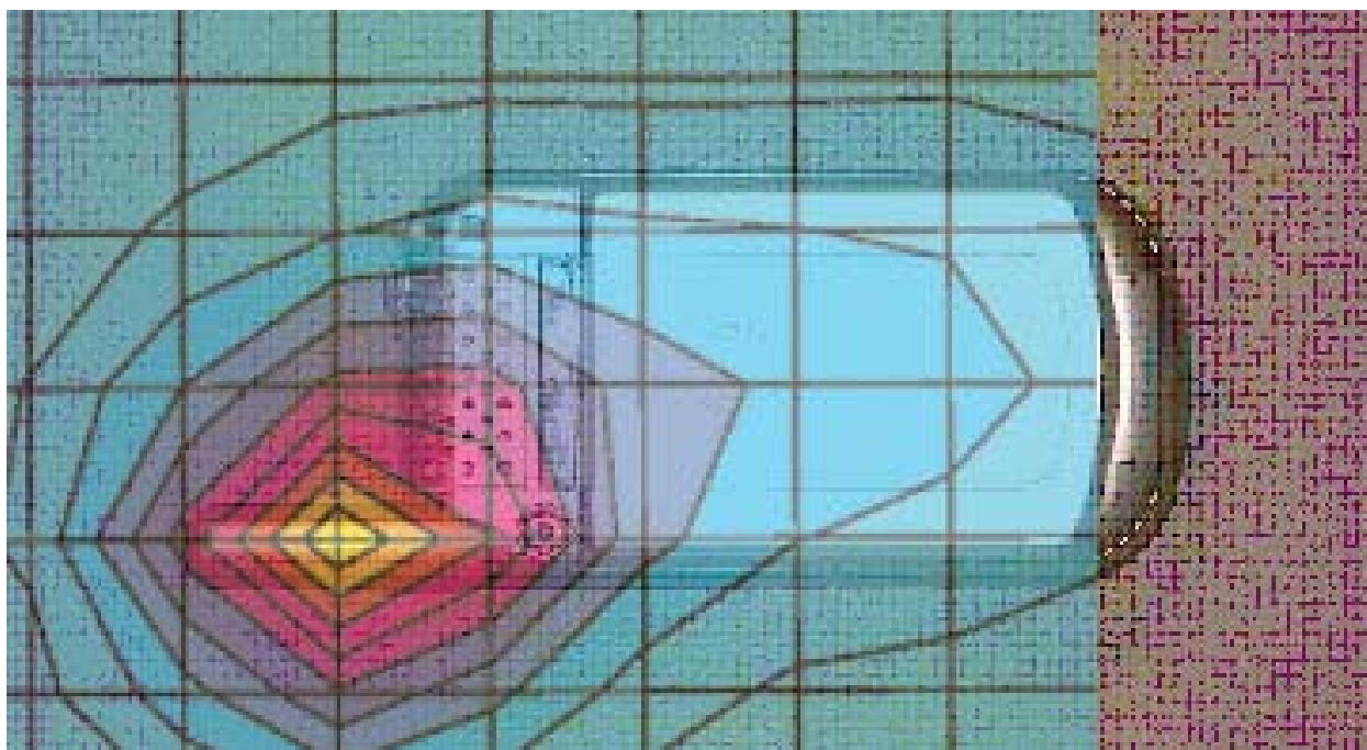
Figure 3. Typical 1900 MHz Body-Worn Contour Overlaid on Phone (GSM Mode)
