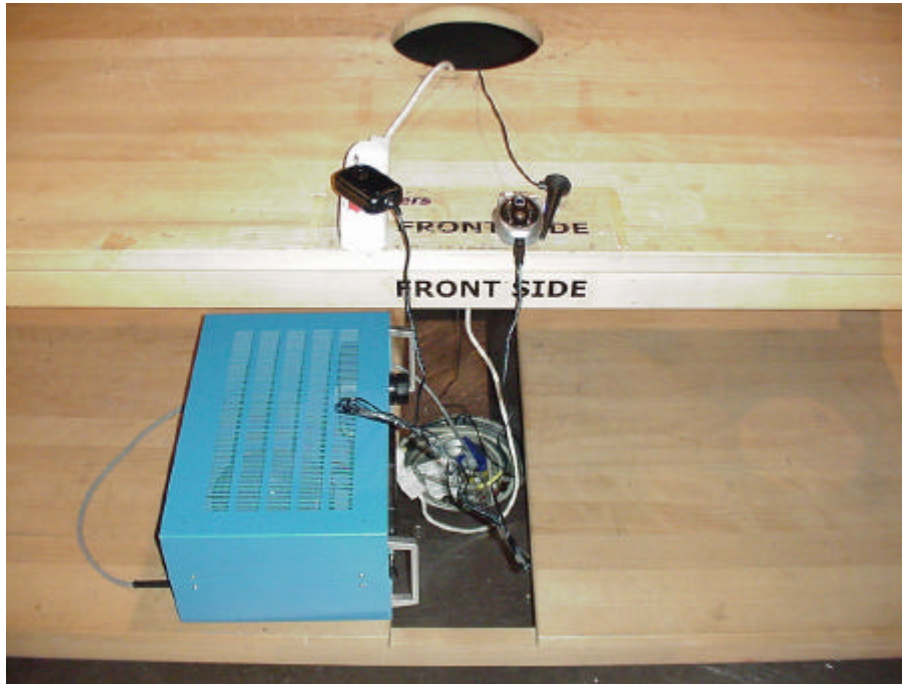
Picture 5 : Setup for radiated emissions tests (< 1 GHz)
