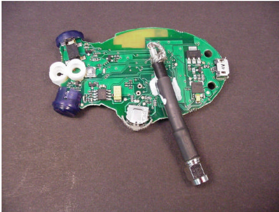
Picture 2 : EUT (view to the PCB top side, incl. temp. antenna connector)
