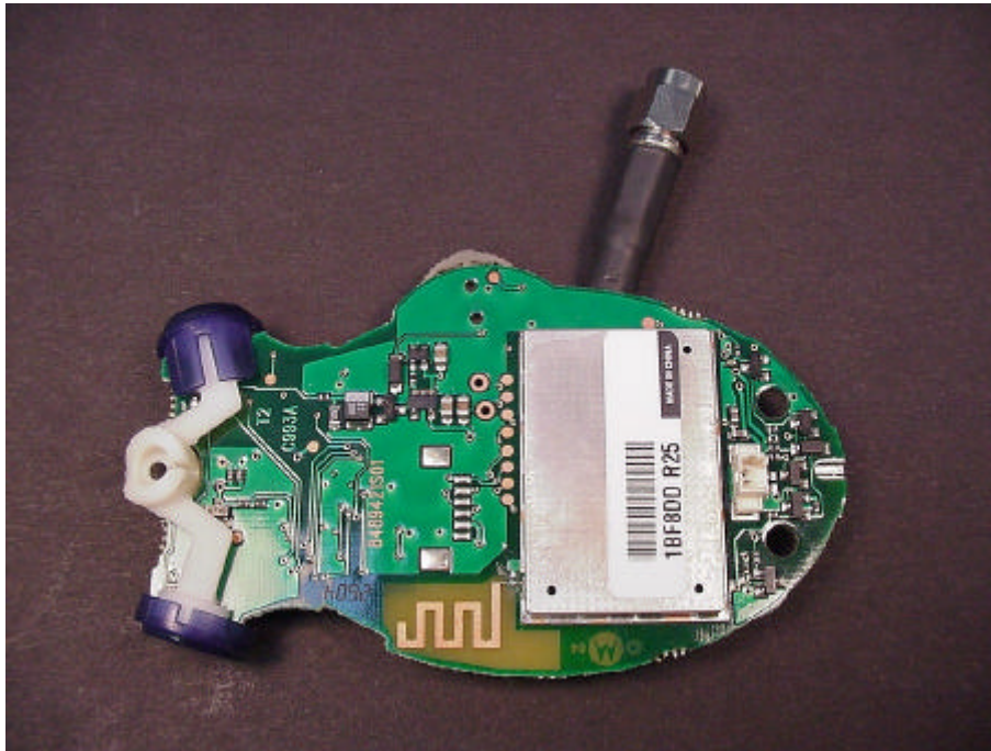
Picture 3 : EUT (view to the PCB bottom side, incl. temp. antenna connector)
