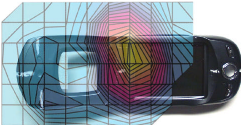
Figure 4. Typical 1900MHz Right Head Adjacent Contour Overlaid on Phone with Antenna Fixed (15 ° Tilt)
