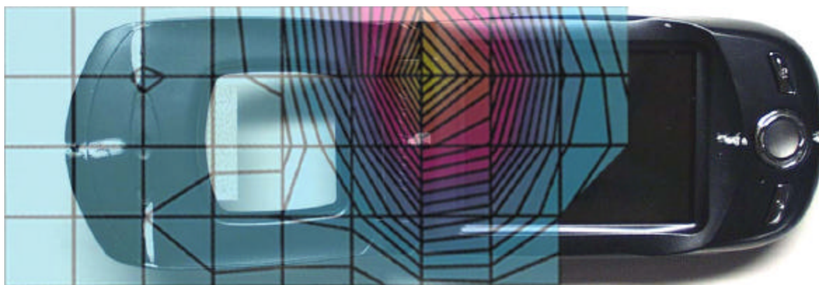
Figure 3. Typical 1900MHz Right Head Adjacent Contour Overlaid on Phone with Antenna Fixed (Cheek Touch)
