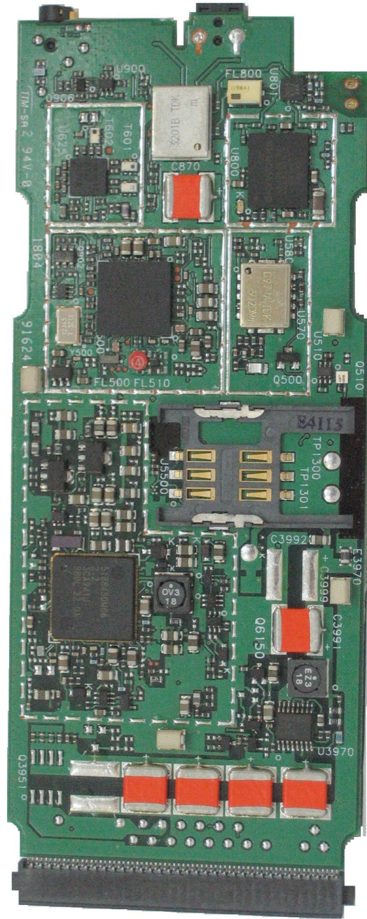
Bottom View (Shields Removed)
