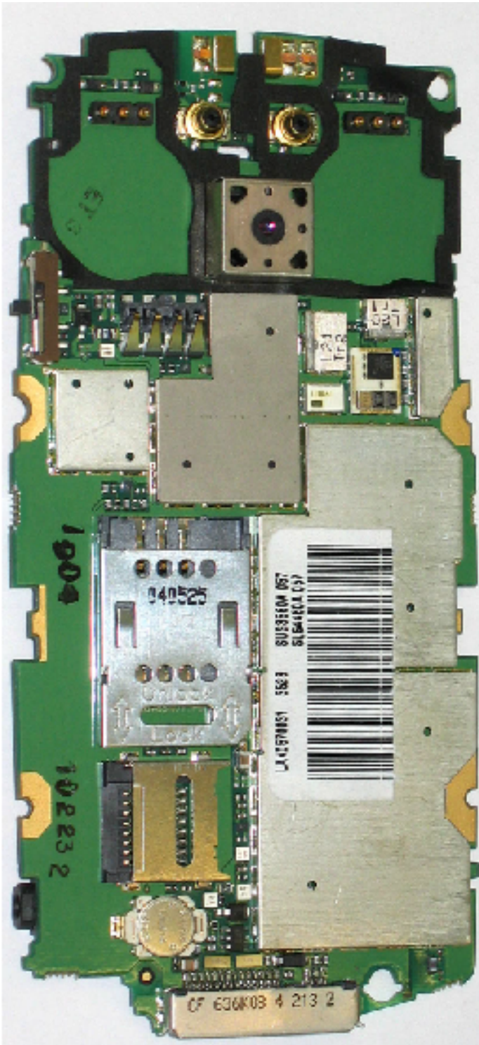
Rear View with Shields
