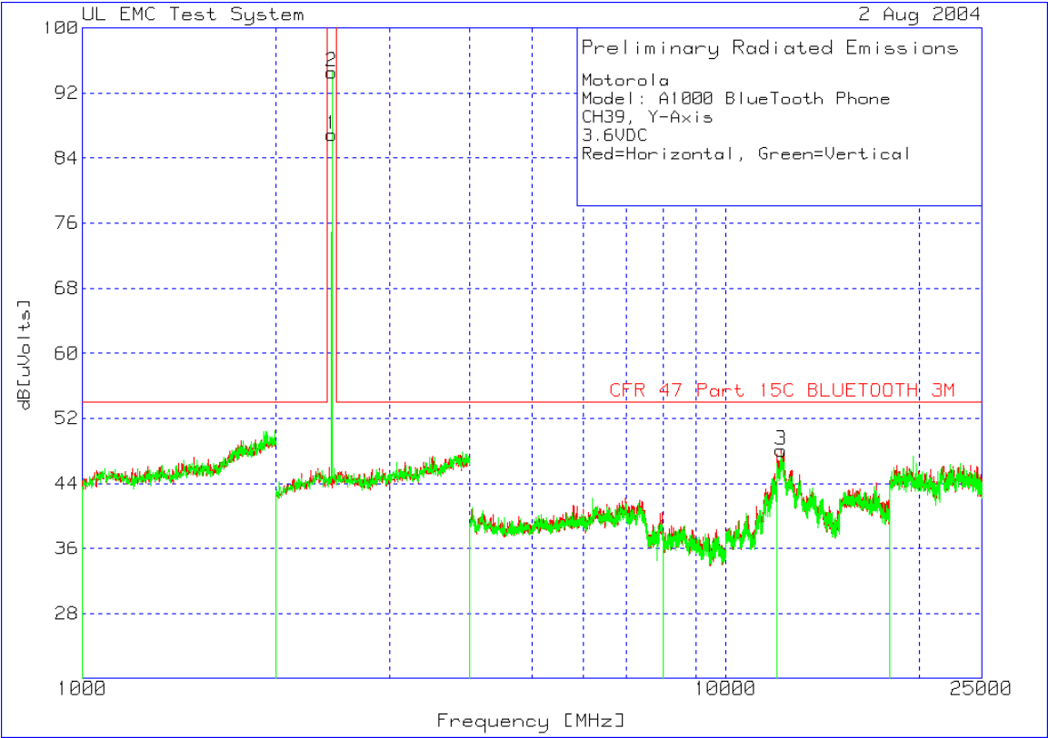
1-25GHz Mid-Channel Y-Orientation
