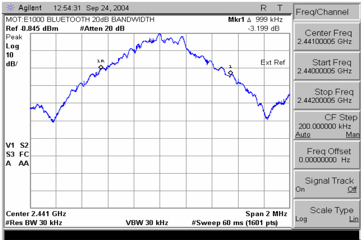
20 dB Bandwidth Plot
