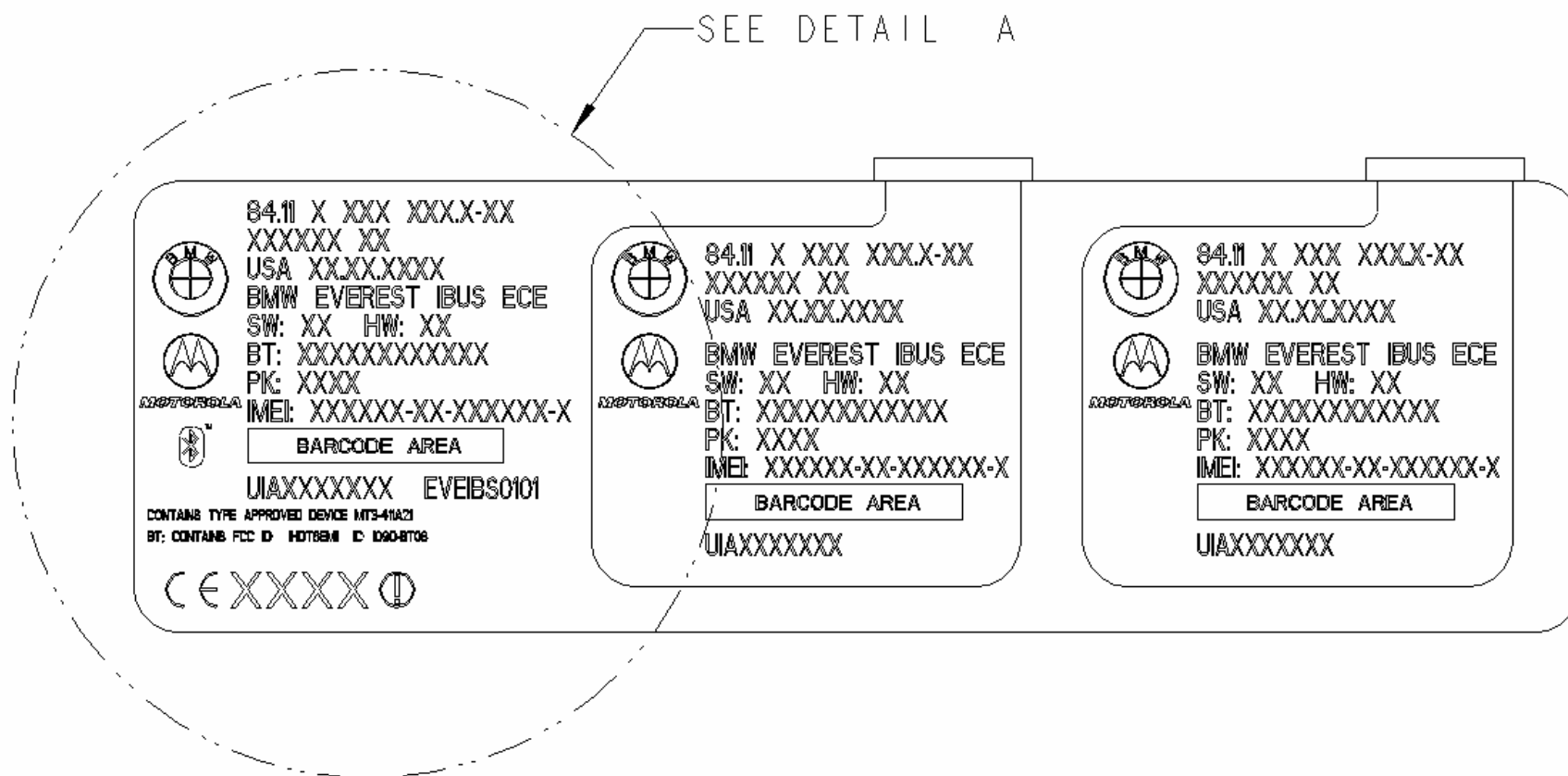
Picture 1. External topside label placed onto the Telecommunication Unit (TCU). FCC ID information is clearly displayed on the label.
