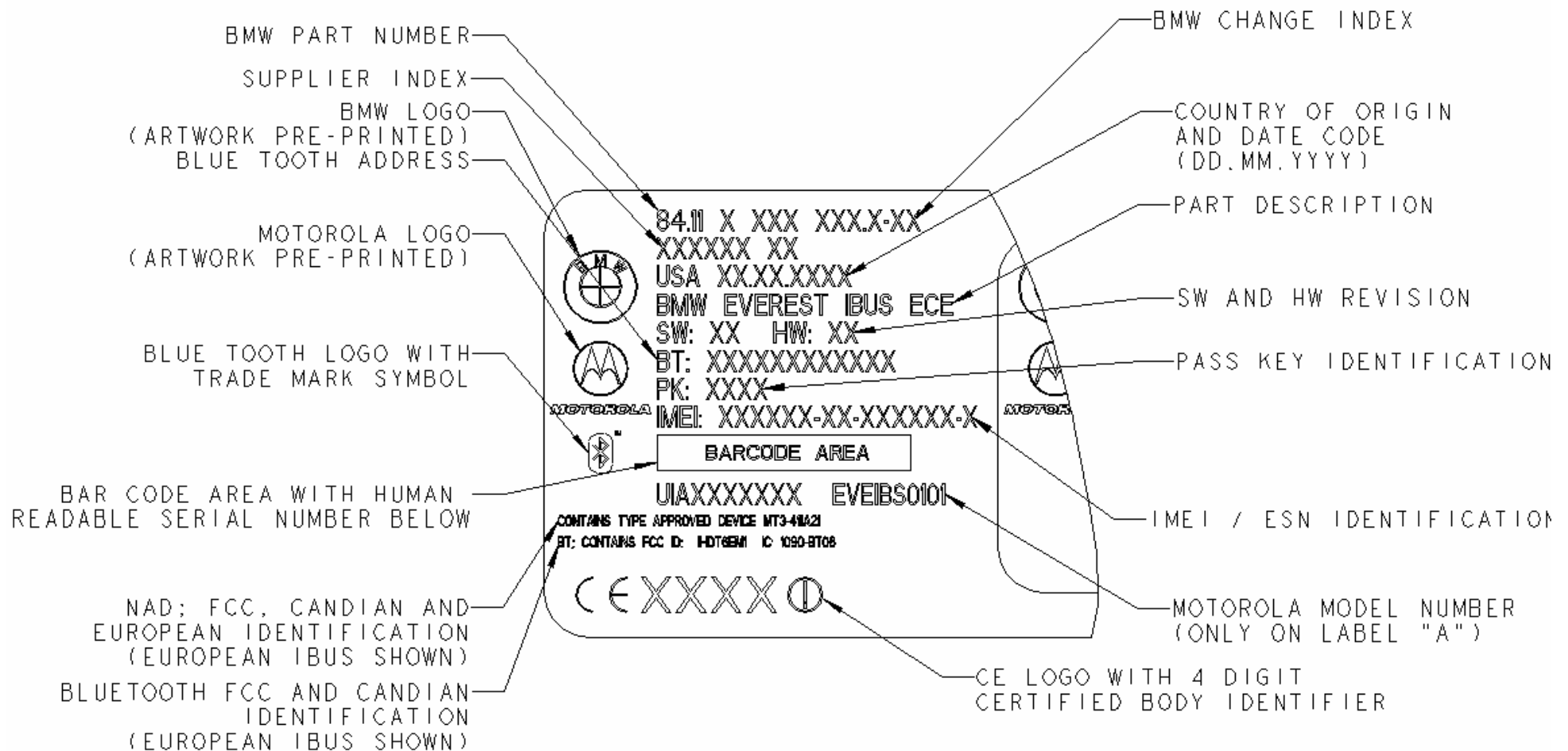
DETAIL A Shown here is IBUS US FCC ID: IHDT6EM1
