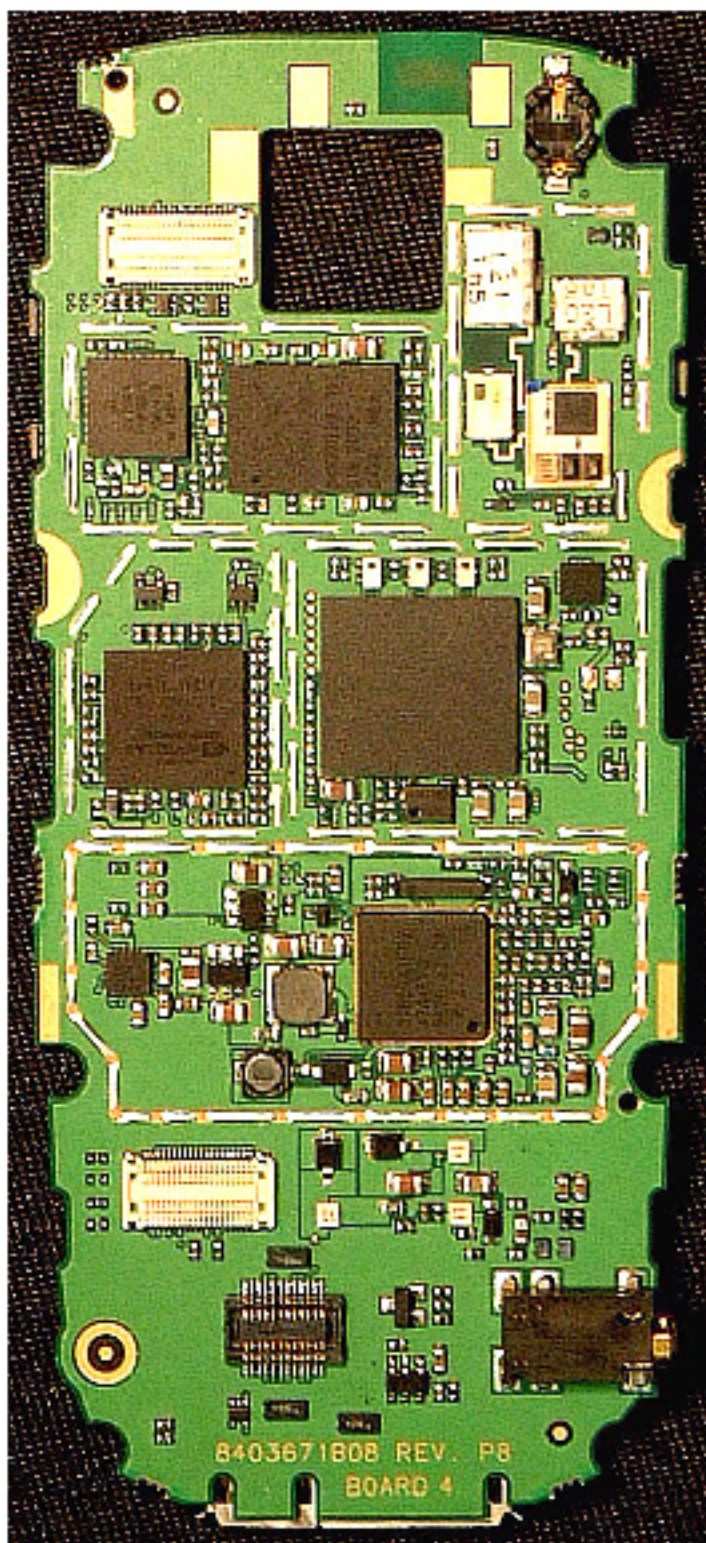
Front View Without Shields
