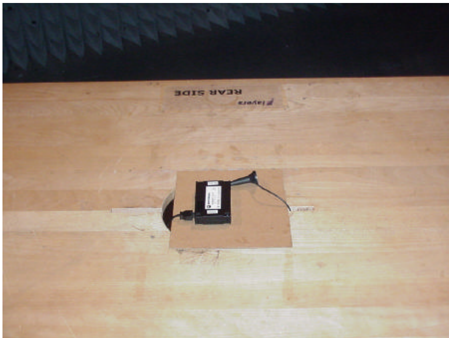
Picture 4 : Setup for radiated emissions tests (< 1 GHz)
