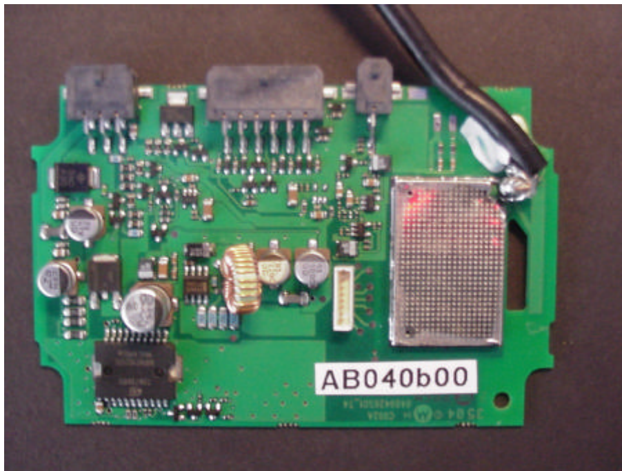
Picture 2 : EUT (view to the PCB top side, incl. RF cable to temp. antenna connector)
