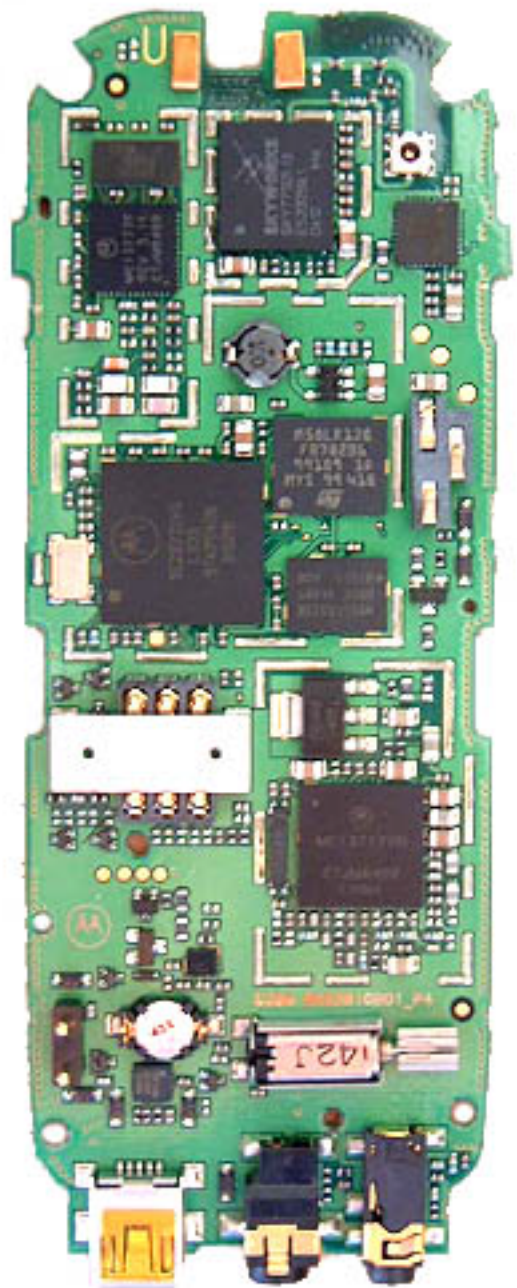
Rear View (Shields Removed)
