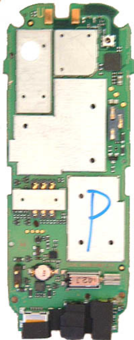
Rear View
