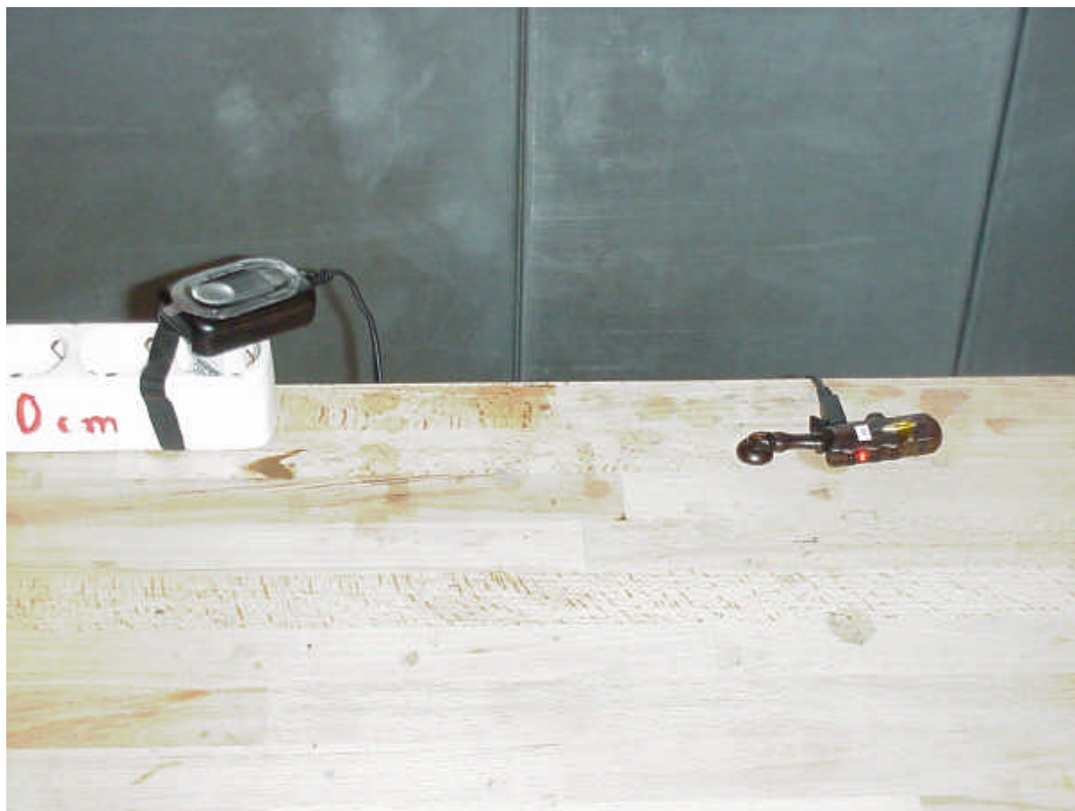
Photo 2: Setup for the test conducted emissions (AC power line)
