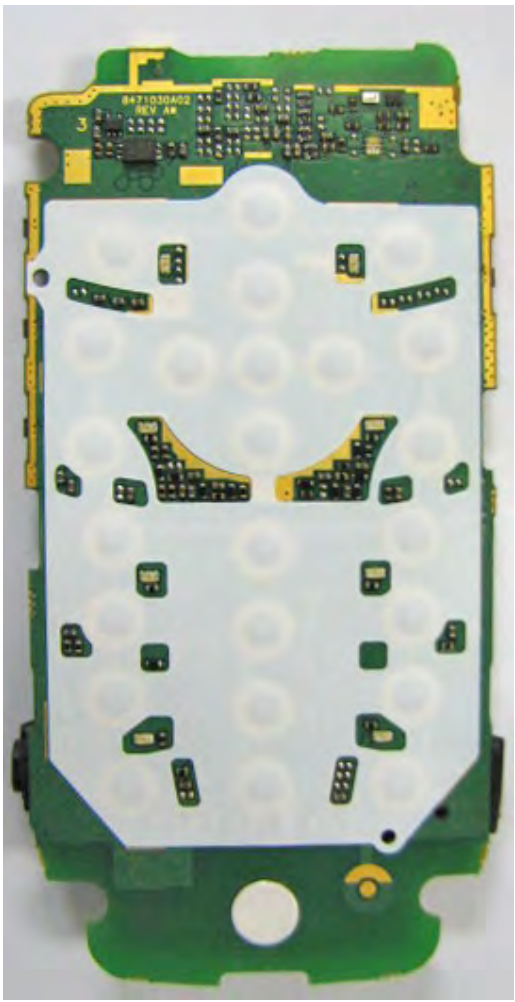
Front View
