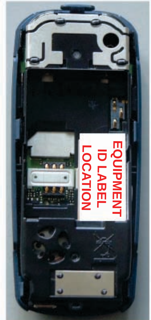
Rear View with Battery Cover removed showing ID Label
