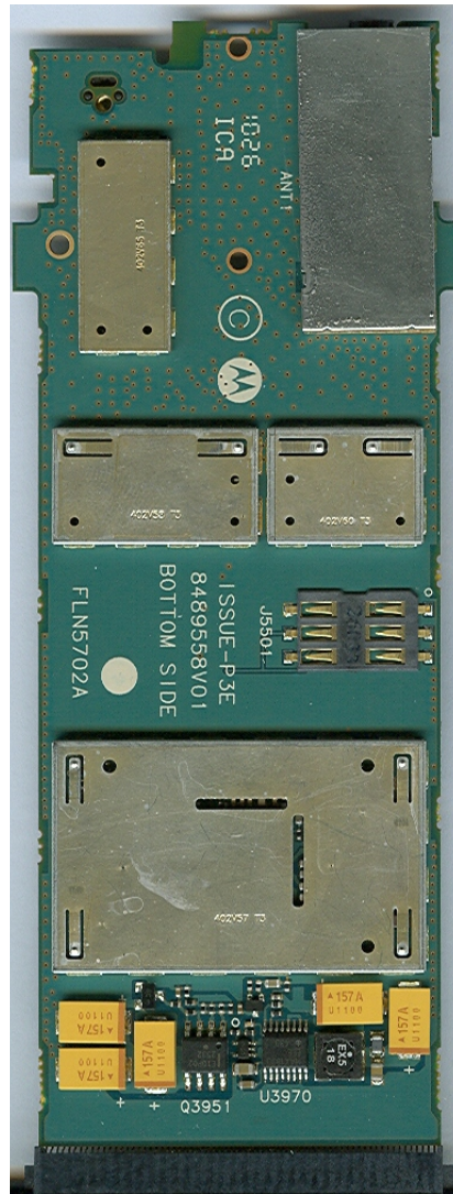
Bottom side view with shields
