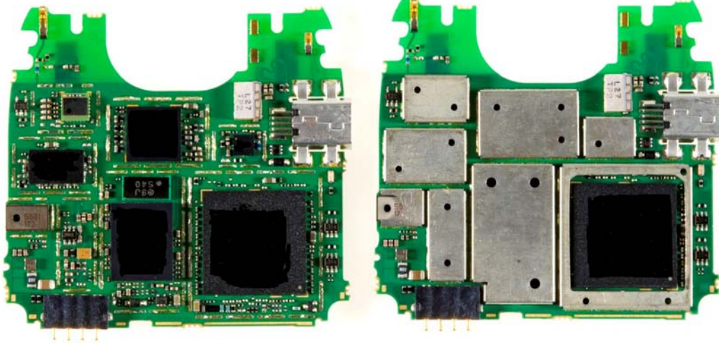
Main Board Side A - Without Shields
