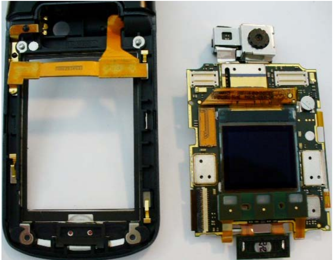
Inside Front Housing
