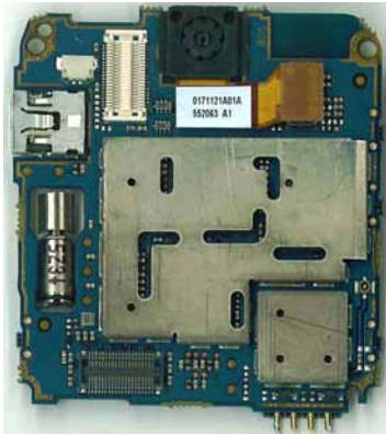
Main PCB (Side A)
