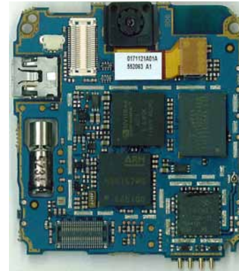
Main PCB (Side A) with shields removed
