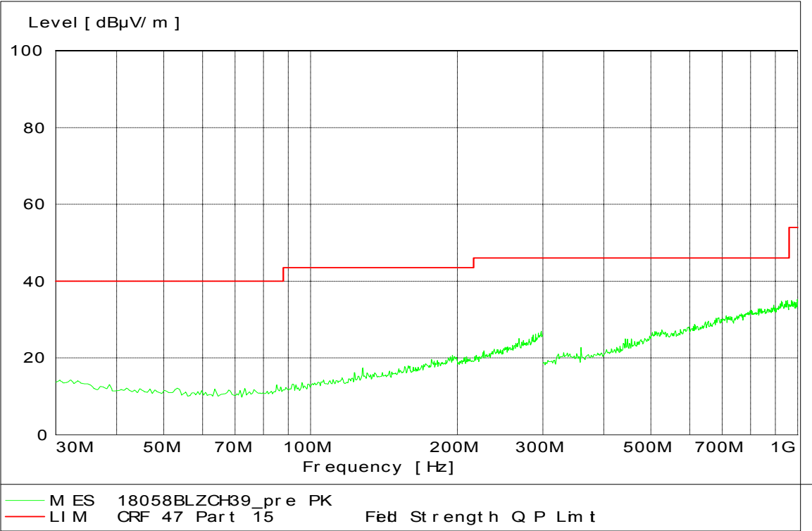
30 -1000 MHz mid Channel Dual Polarization Z
