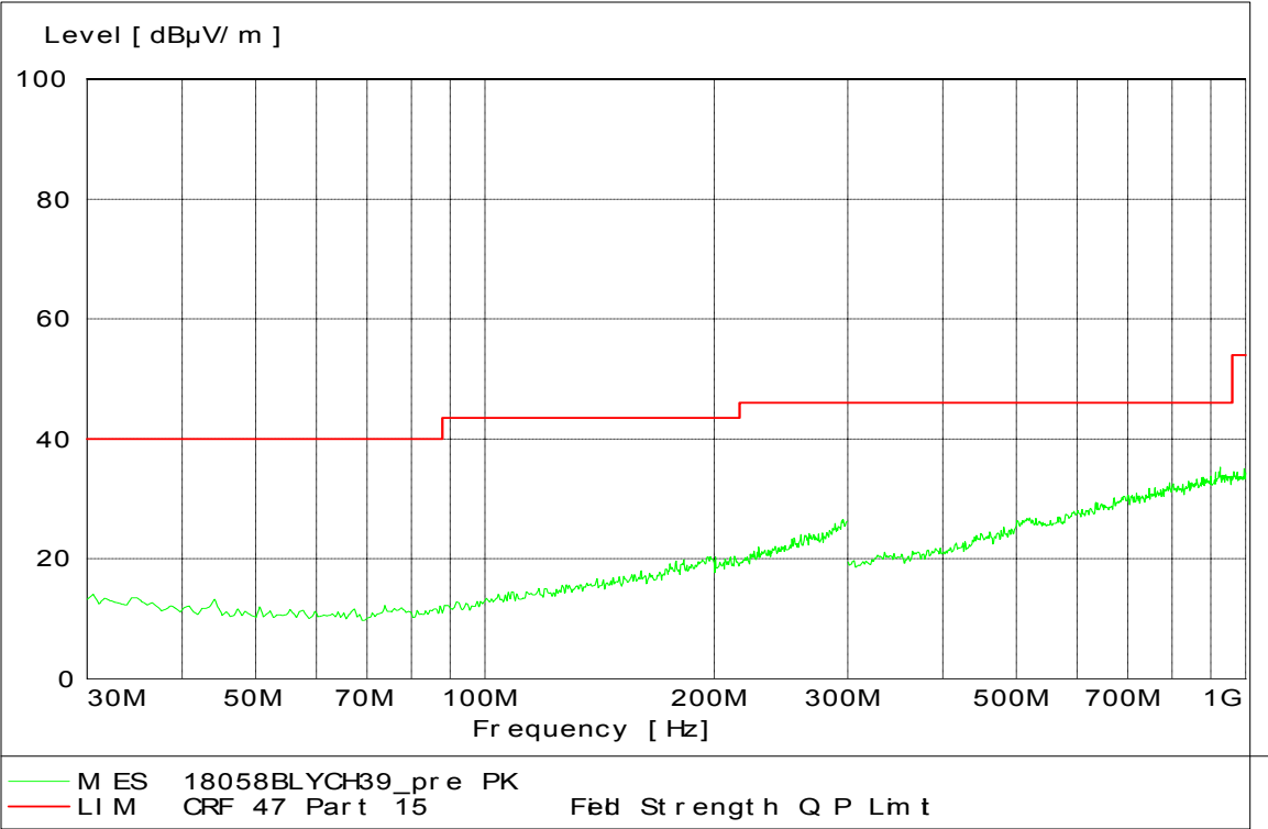
30 -1000 MHz Mid Channel Dual Polarization Y
