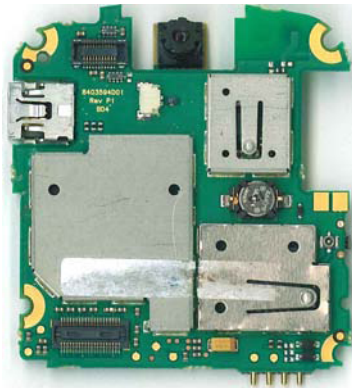
Main PCB (Side B)
