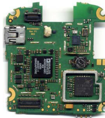
Main PCB (Side B) with shields removed
