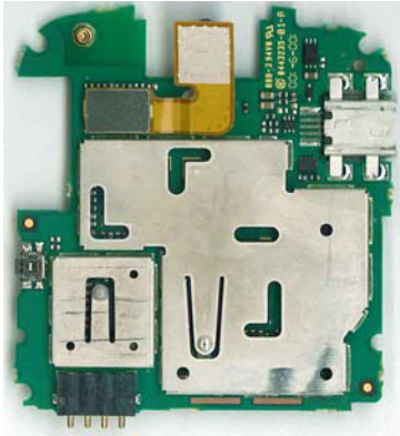
Main PCB (Side A)
