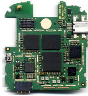
Main PCB (Side A) with shields removed
