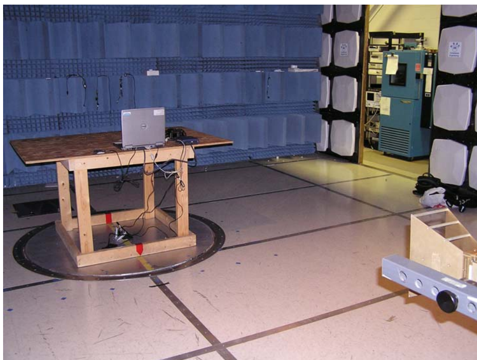
Figure 2. Part 15 Radiated Emissions Measurement Setup
