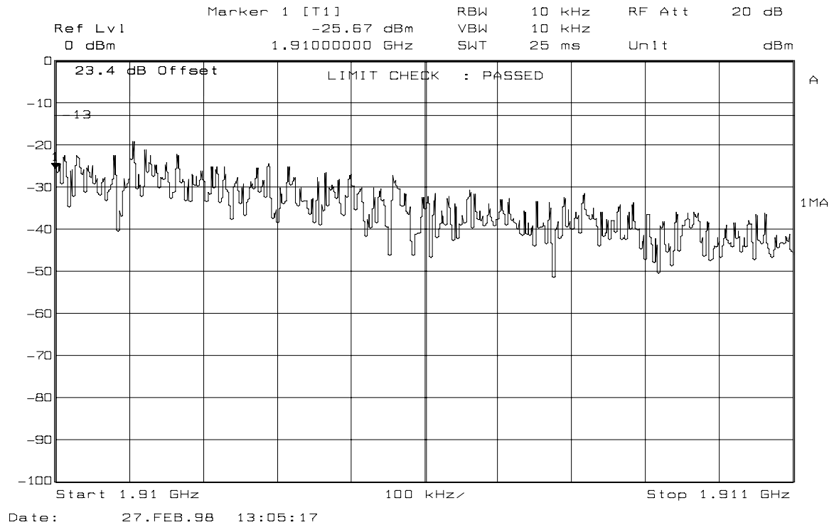
Figure 13.4: Carrier 1908.75 MHz, Spectrum 1910 MHz to 1911 MHz
