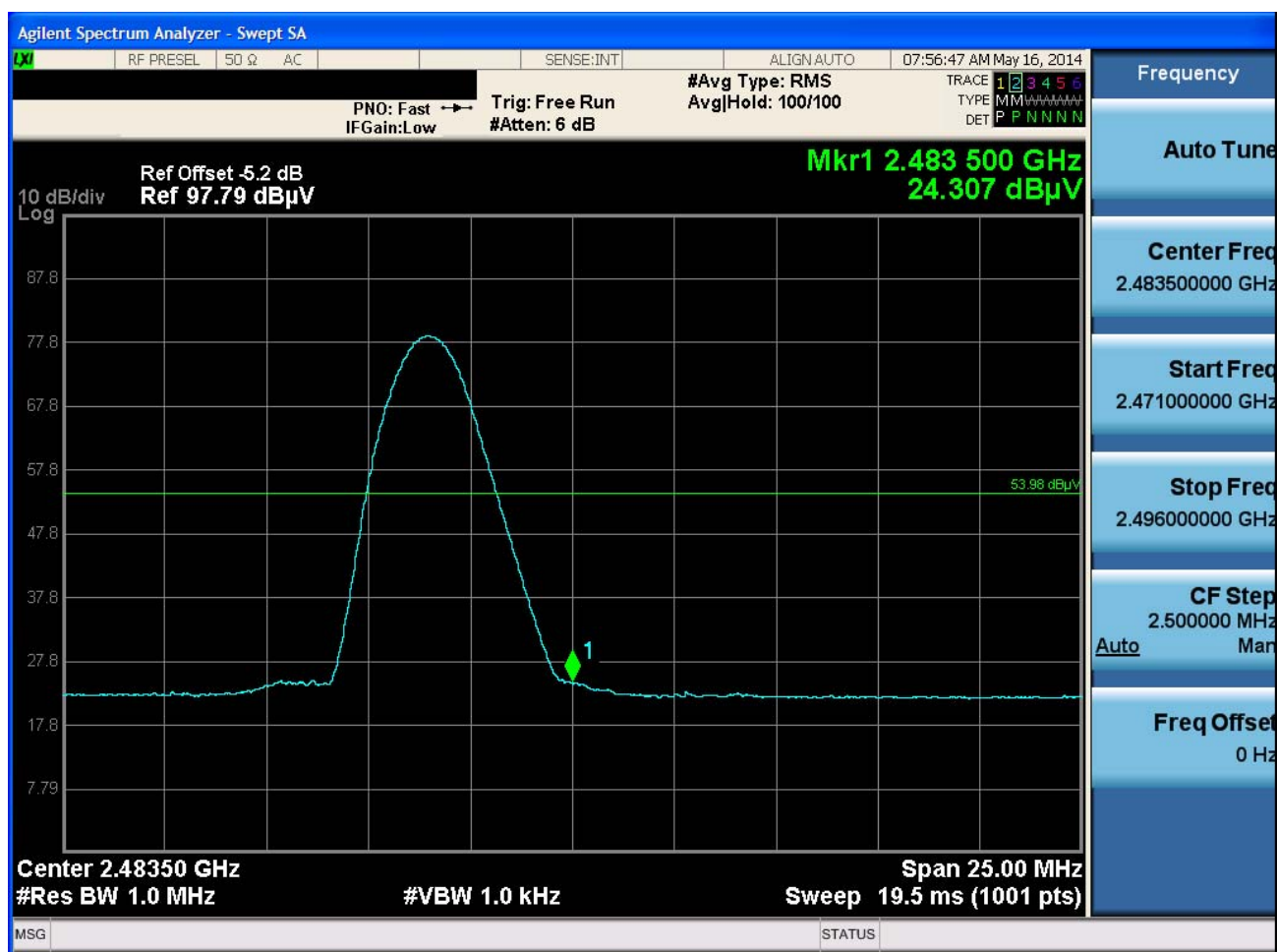
Plot 6-44. Radiated Restricted Upper Band Edge Measurement with WCP (Average)
