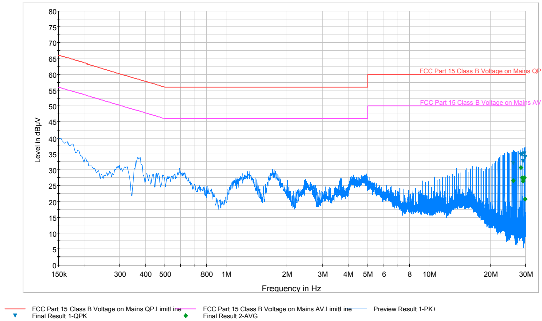
Plot 6-46. Line-Conducted Test Plot (L1)
