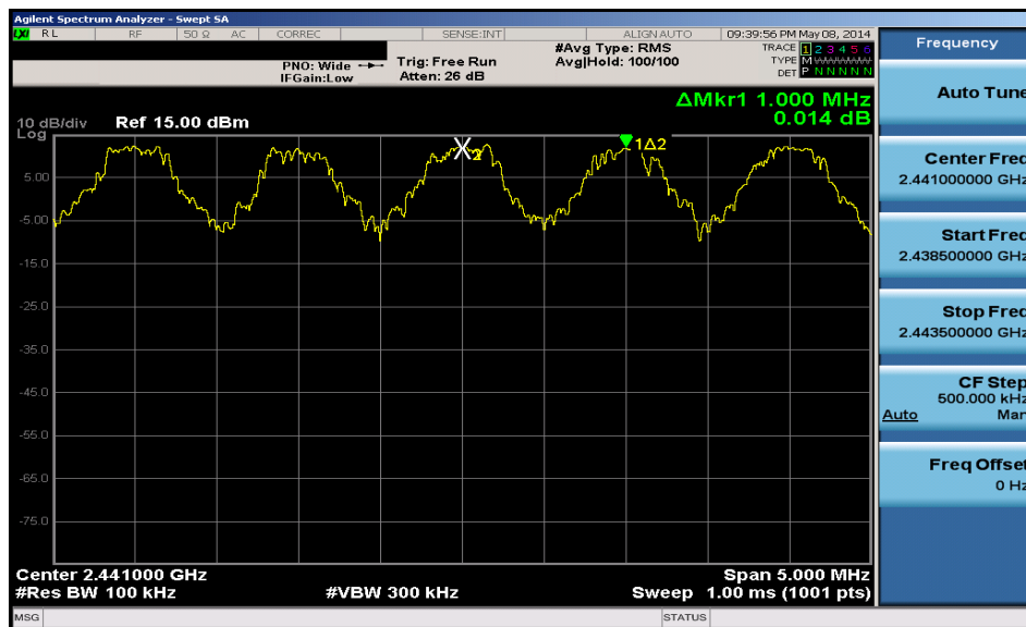
Plot 6-32. Channel Spacing Plot (Bluetooth)
