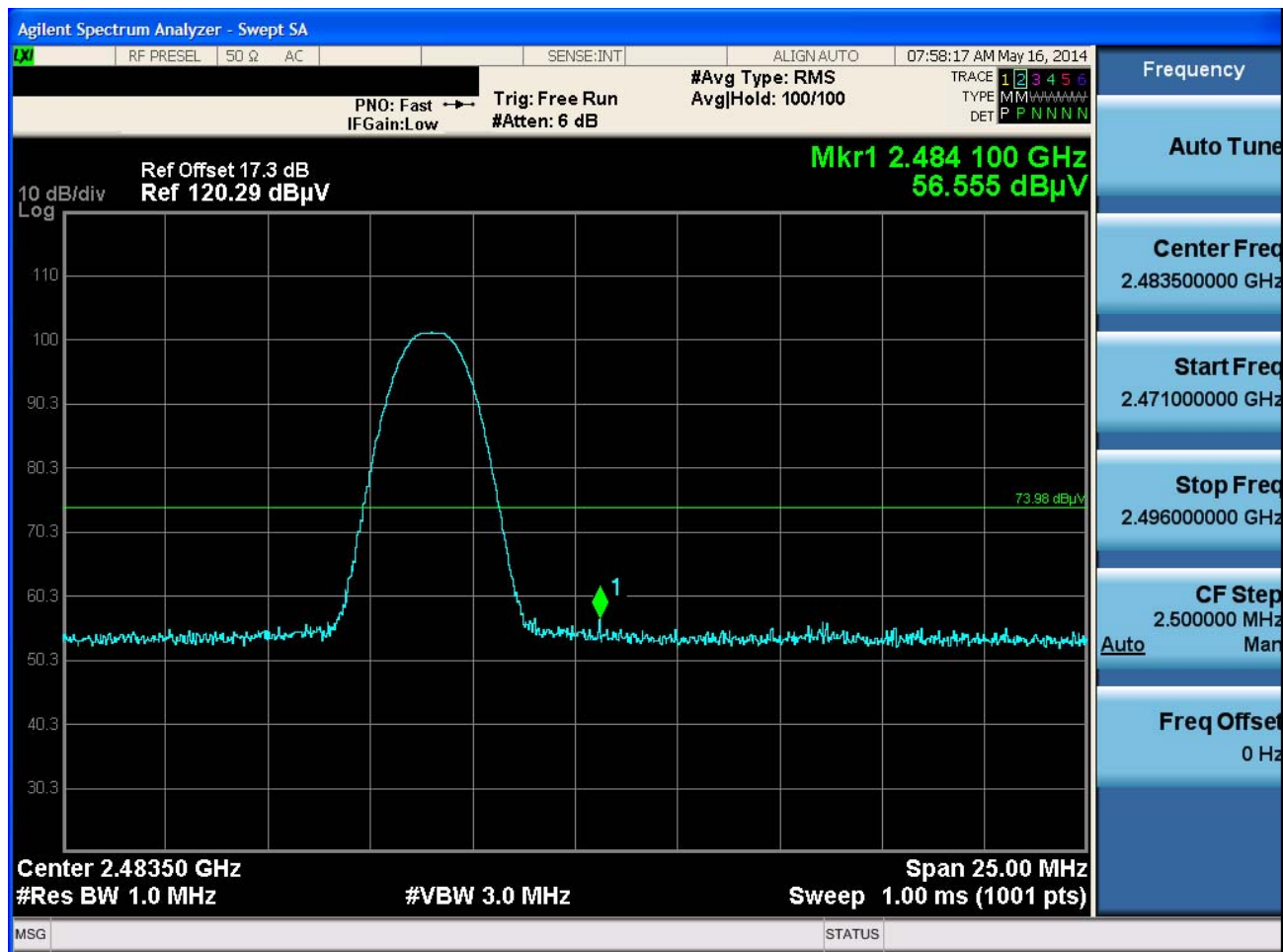
Plot 6-45. Radiated Restricted Upper Band Edge Measurement with WCP (Peak)
