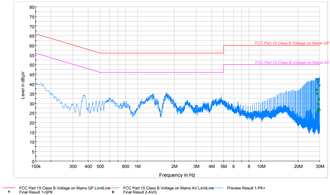
Plot 6-47. Line-Conducted Test Plot (N)
