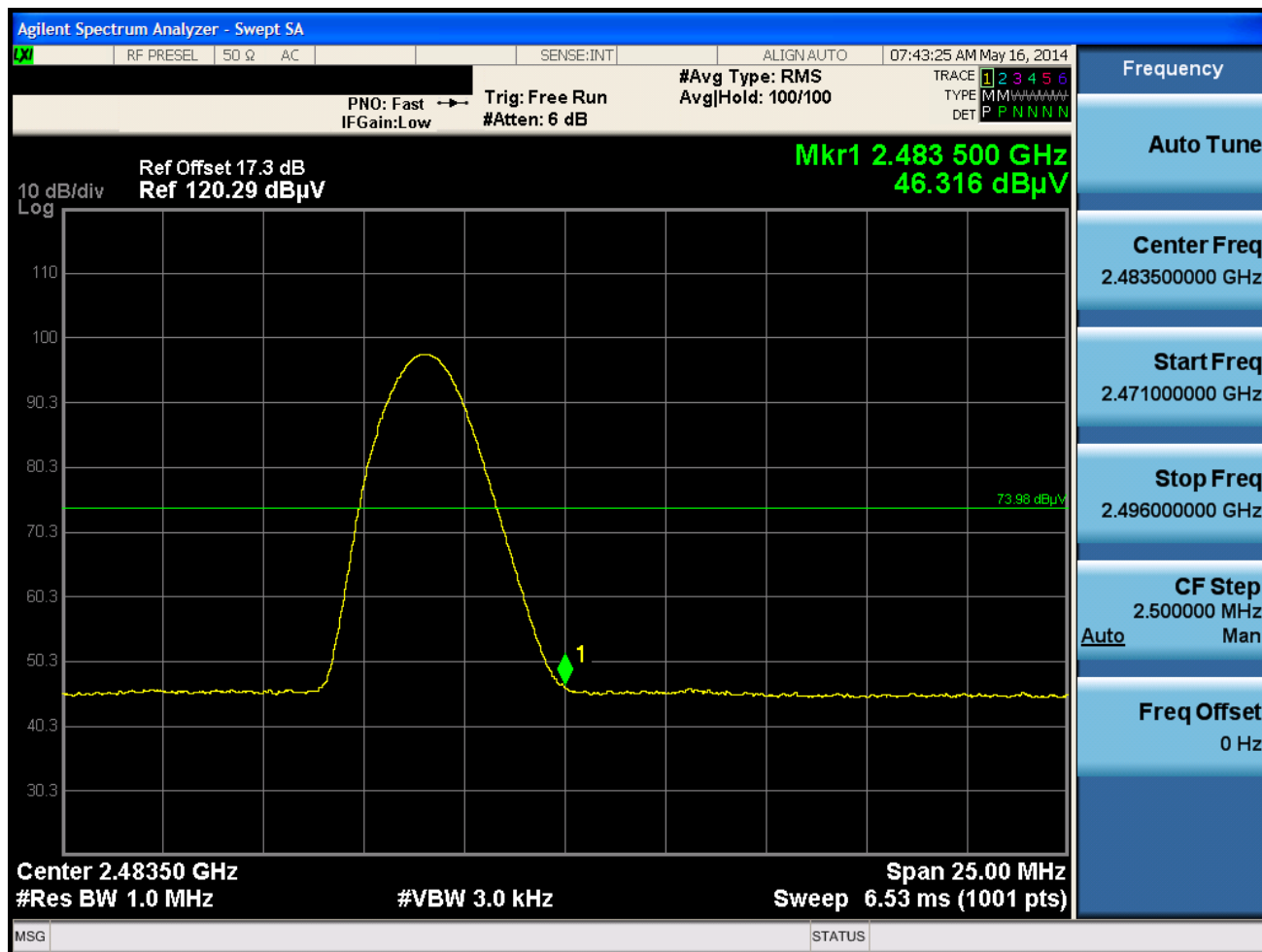
Plot 6-20. Radiated Restricted Upper Band Edge Measurement with WCP (Average)
