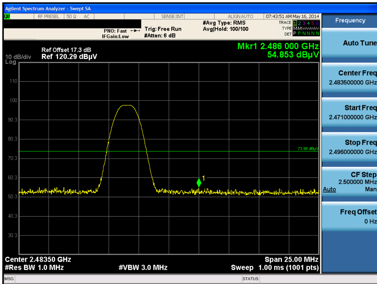
Plot 6-21. Radiated Restricted Upper Band Edge Measurement with WCP (Peak)
