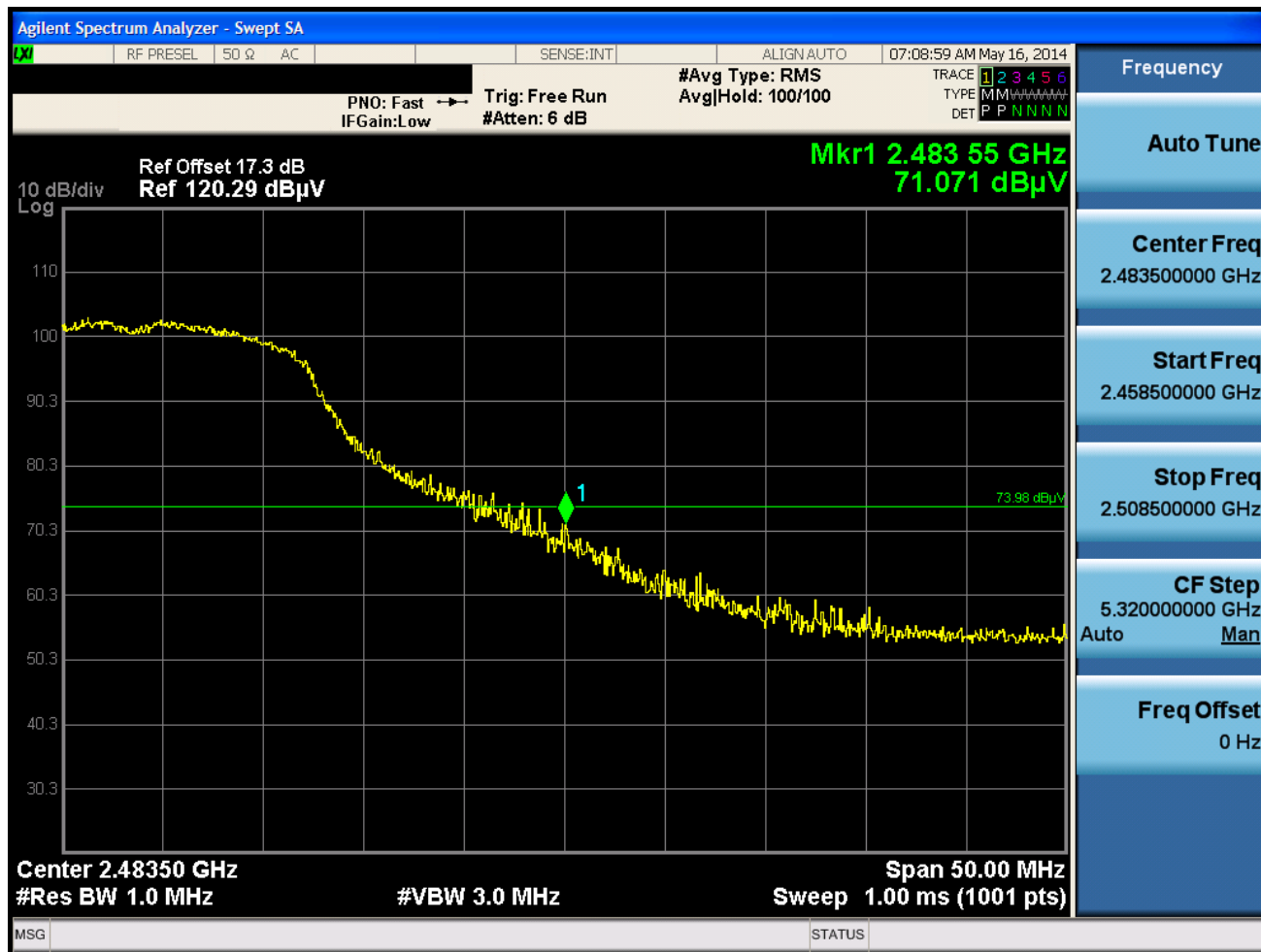
Plot 6-36. Radiated Restricted Band Edge Measurement with WCC (Peak)
