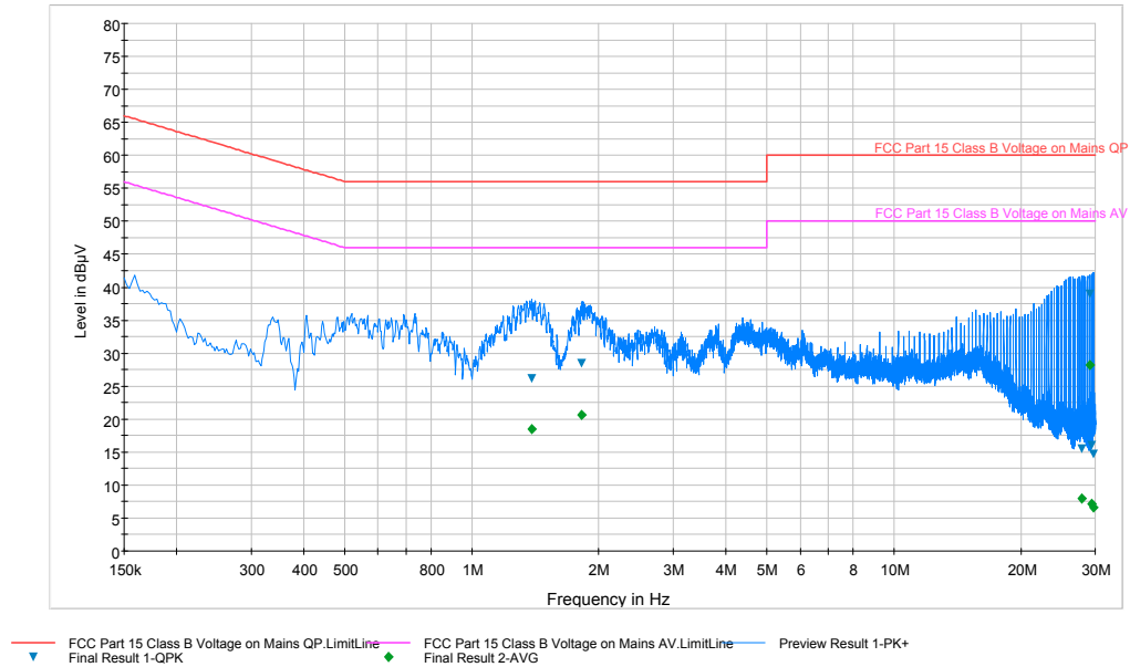
Plot 6-38. Line Conducted Plot with 802.11b (N)
