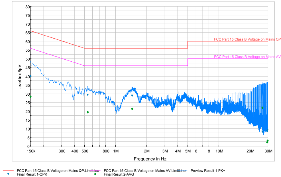
Plot 6-37. Line Conducted Plot with 802.11b (L1)
