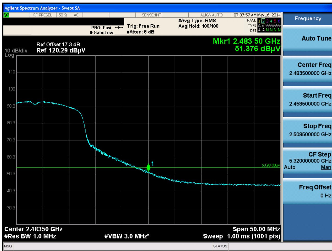
Plot 6-35. Radiated Restricted Band Edge Measurement with WCC (Average)
