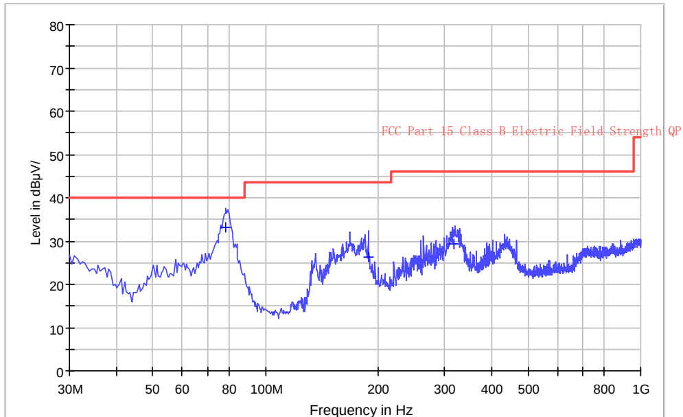
Electric Field Strength FCC 15
