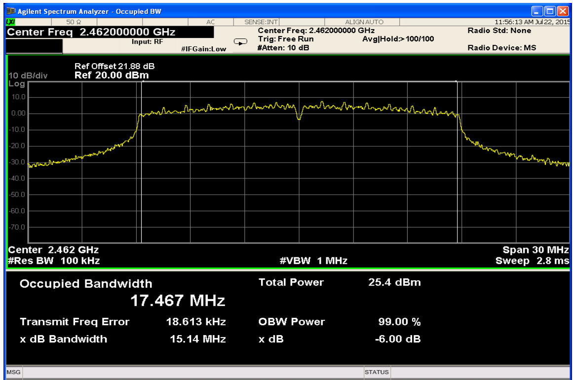
6dB Bandwidth Channel 11 @ 28.9 Mbps
