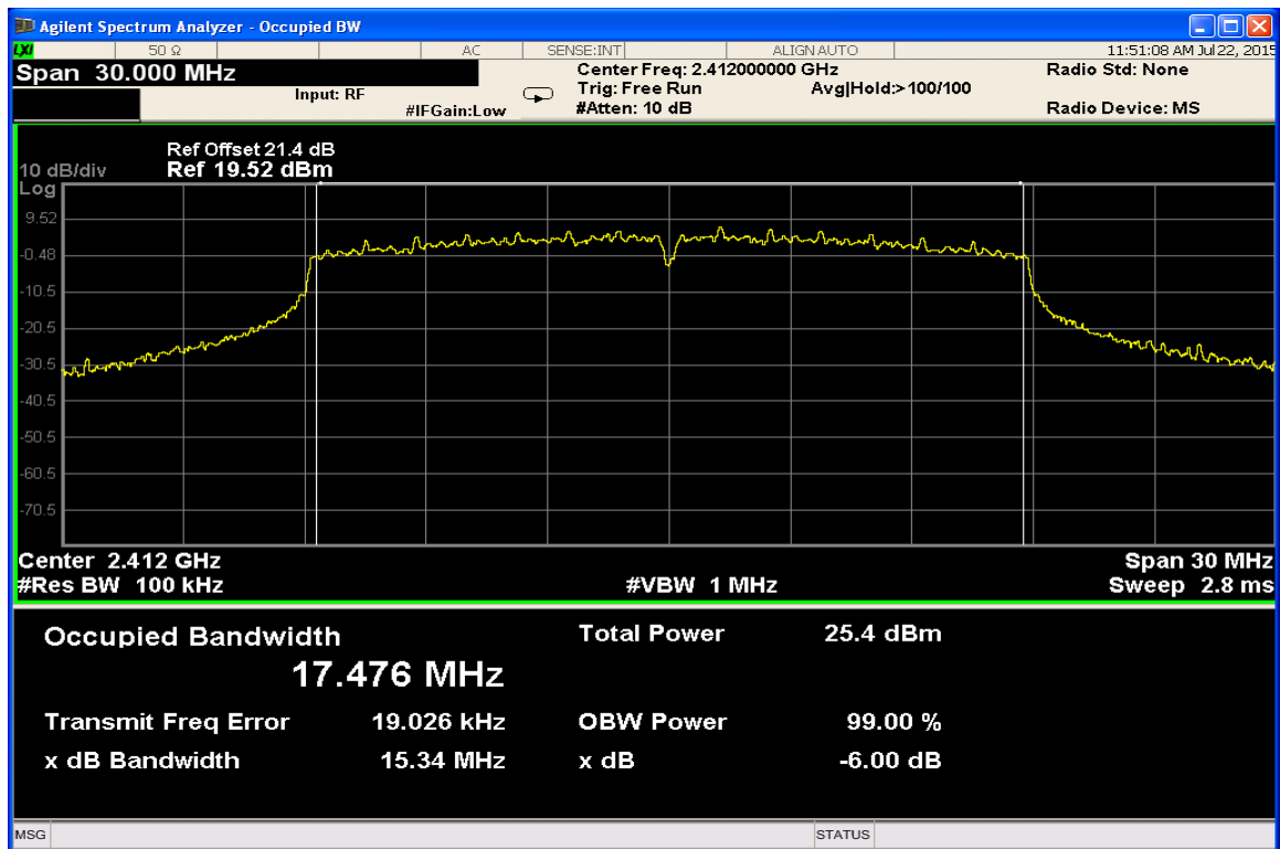
6dB Bandwidth Channel 1 @ 28.9 Mbps
