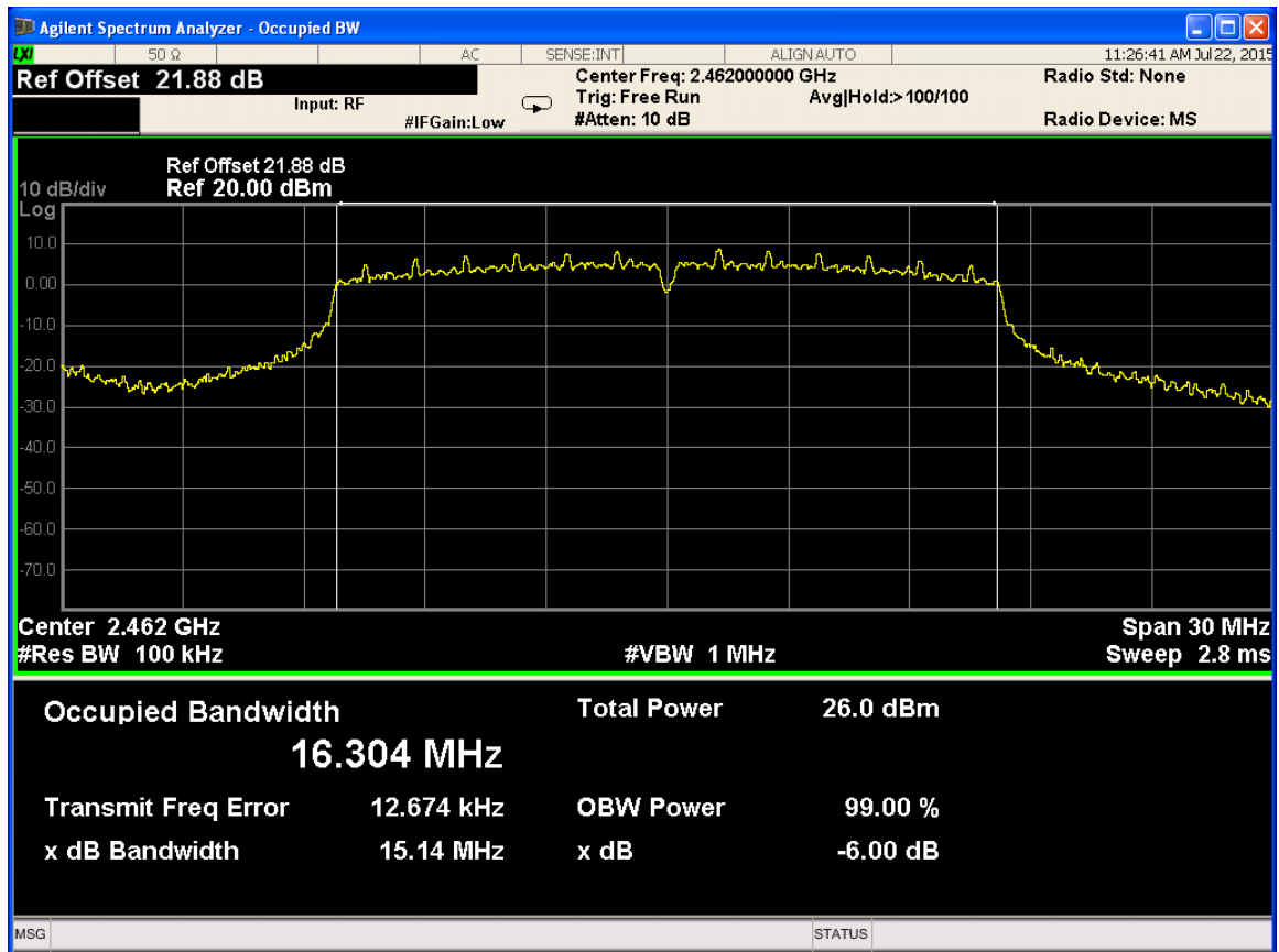
6dB Bandwidth Channel 11 @ 18 Mbps
