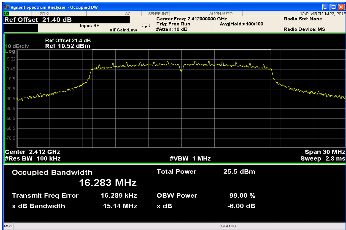
6dB Bandwidth Channel 1 @ 18 Mbps
