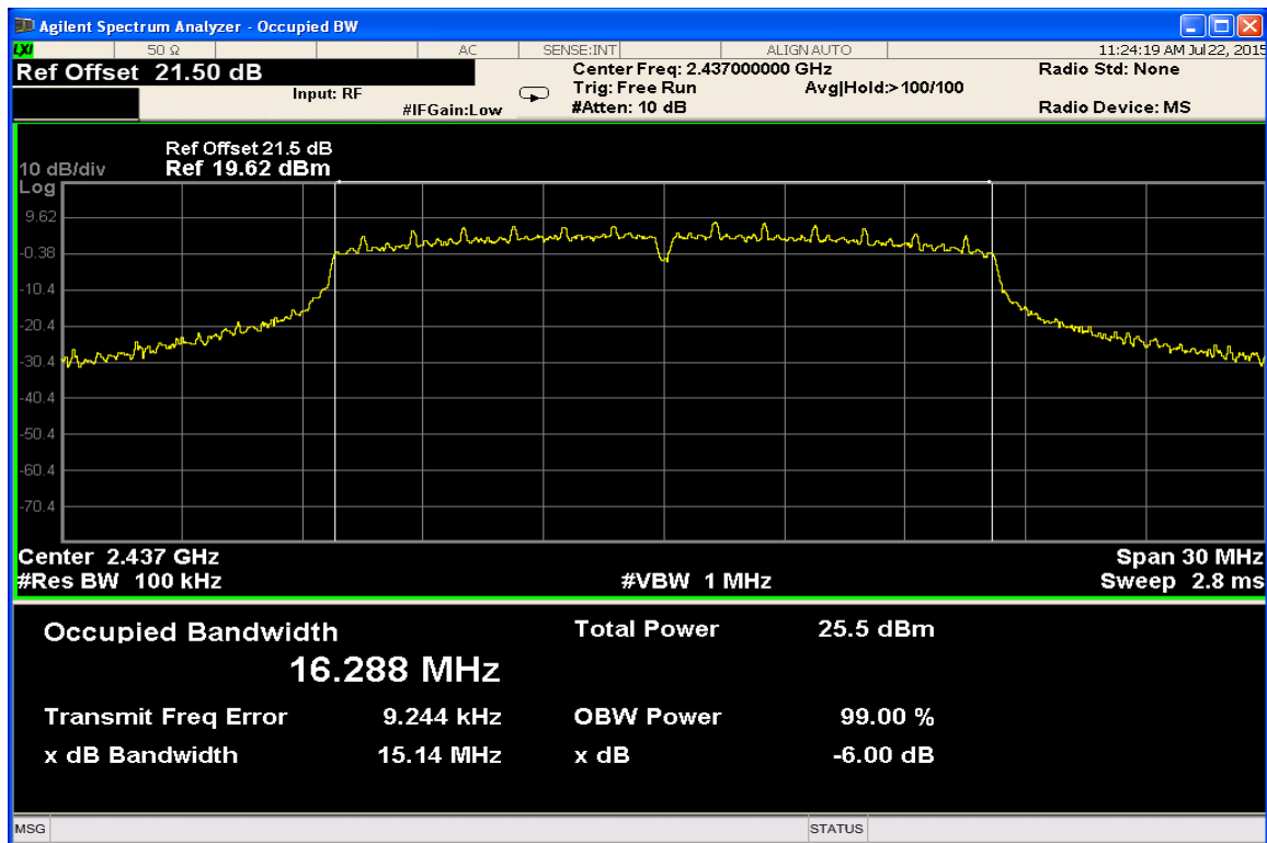
6dB Bandwidth Channel 6 @ 18 Mbps
