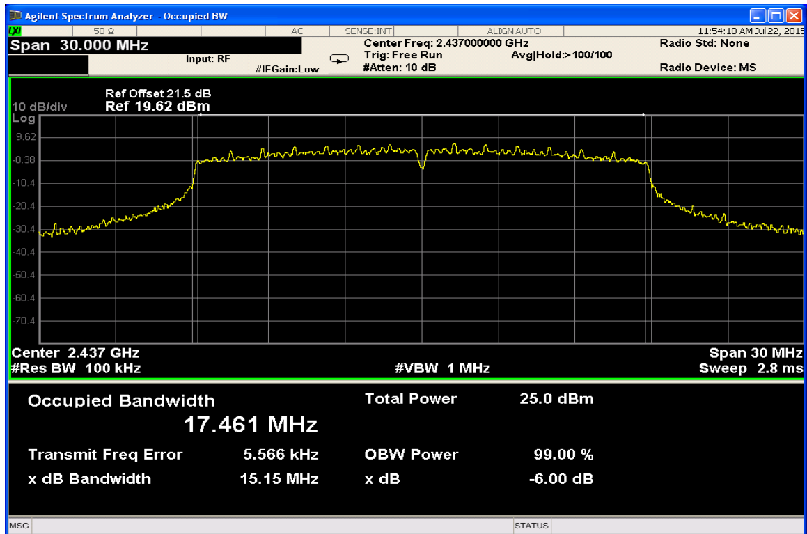
6dB Bandwidth Channel 6 @ 28.9 Mbps
