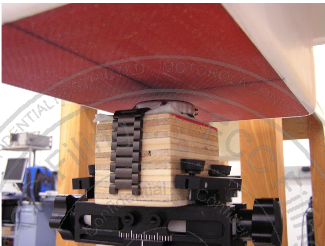
Figure 13: Front of Large Body Device (with Metal band) against Phantom
