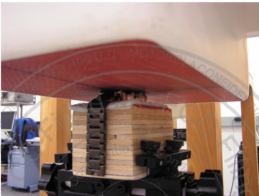
Figure 9: Back of Small Body Device (with Metal band) against Phantom
