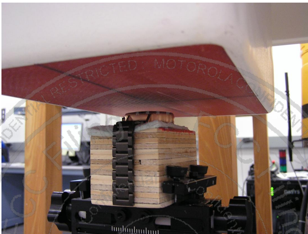
Figure 17: Front of Small Body Device (with Metal band) against Phantom
