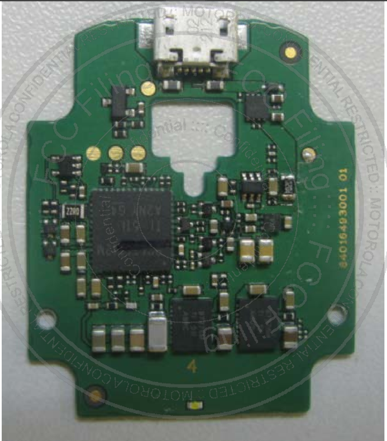
Photograph 9-1: Front side view of the device's PC Board.
