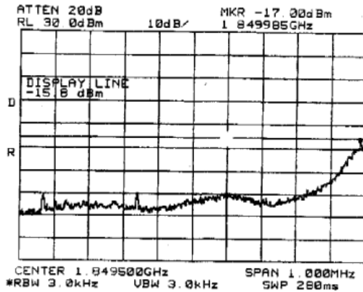
Figure 10.2: Carrier 1850.2 MHz, Spectrum 1849 to 1850MHz.
