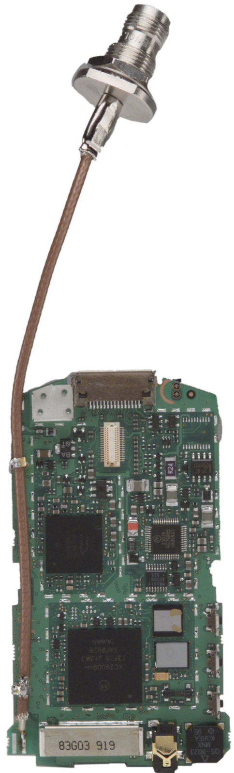
Transceiver Board Rear View (Shields Removed)
