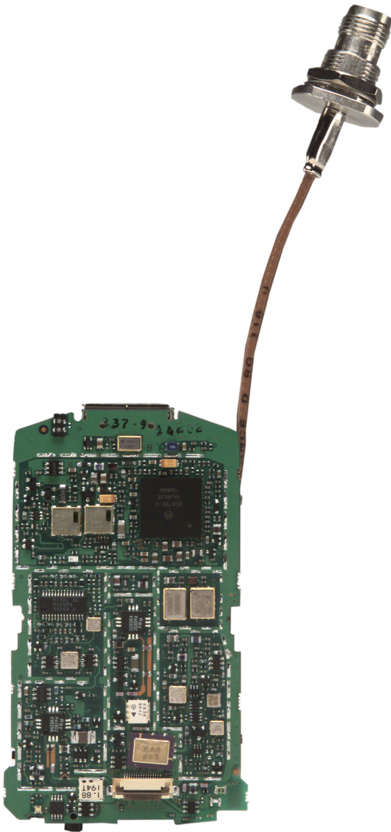
Transceiver Board Front View (Shields Removed)
