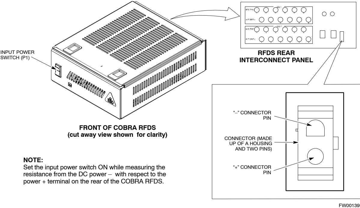
Figure 2-7: DC Distribution Pre-test (COBRA RFDS Detail)
